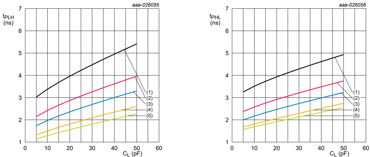
a. LOW to HIGH propagation delay (A to B); V CC(A) = 3.3 V b. HIGH to LOW propagation delay (A to B); V CC(A) = 3.3 V (1) V CC(B) = 1.2 V (2) V CC(B) = 1.5 V (3) V CC(B) = 1.8 V (4) V CC(B) = 2.5 V (5) V CC(B) = 3.3 V
