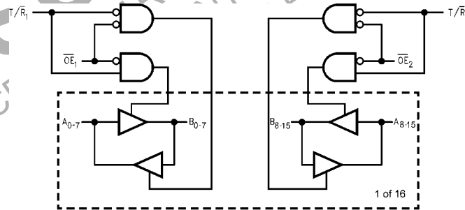
Figure 3. Logic Diagram
