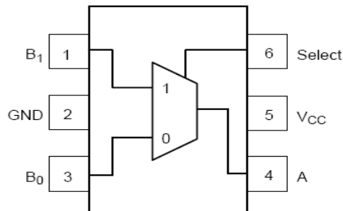
SC70-6 /SOT23-6
