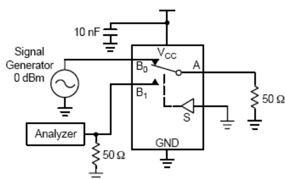
Figure 5 Crosstalk
