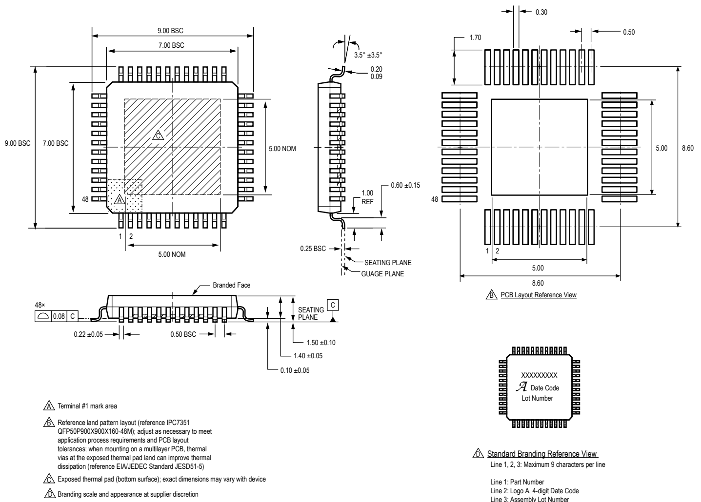
Figure 15: JP Package, 48-Pin LQFP with Exposed Thermal Pad
