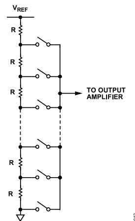
Figure 41. Resistor String Structure
