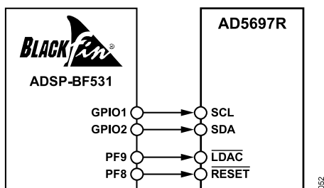
Figure 50. ADSP-BF531 Interface to the AD5338R
