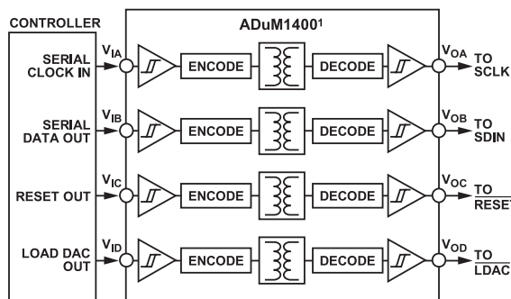
Figure 52. Isolated Interface
