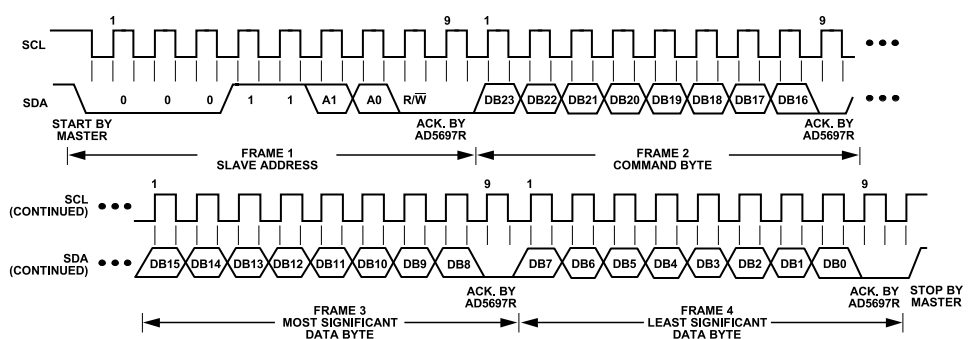
Figure 43. I 2 C Write Operation
