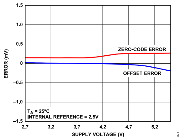
Figure 19. Zero-Code Error and Offset Error vs. Supply Voltage
