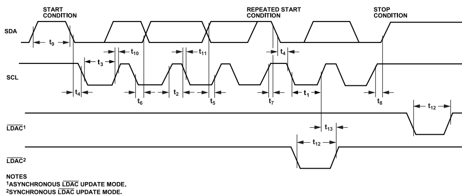
Figure 2. 2-Wire Serial Interface Timing Diagram
