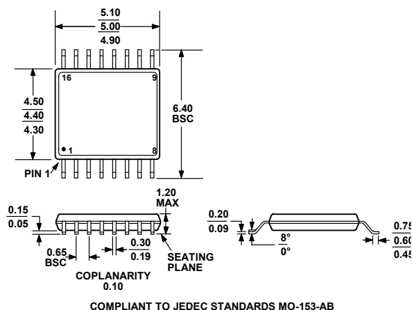
Figure 54. 16-Lead Thin Shrink Small Outline Package [TSSOP] (RU-16) Dimensions shown in millimeters
