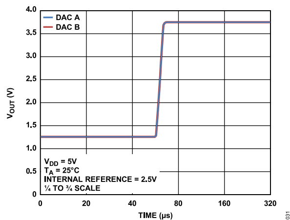
Figure 29. Settling Time
