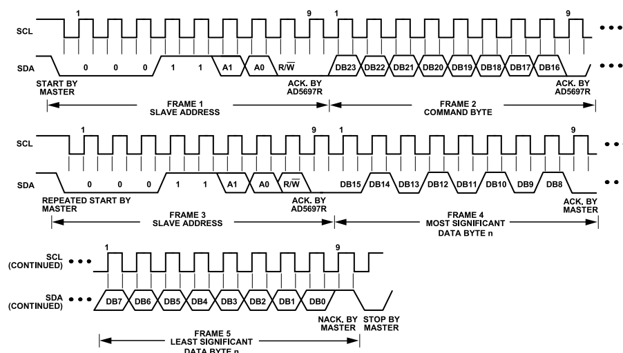
Figure 44. I 2 C Read Operation
