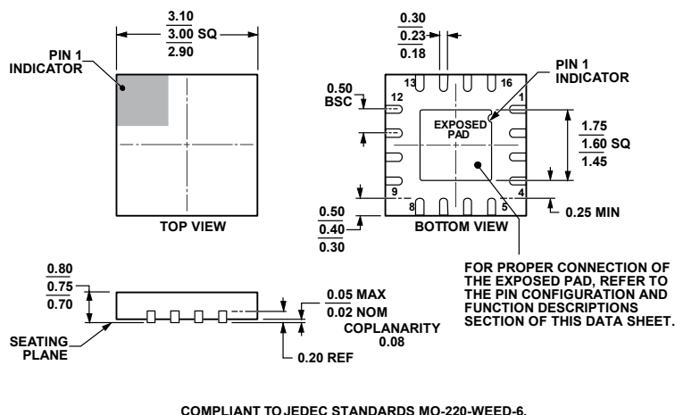
Figure 53. 16-Lead Lead Frame Chip Scale Package [LFCSF] 3 mm × 3 mm Body and 0.75 mm Package Height (CP-16-22) Dimensions shown in millimeters
