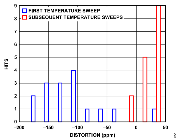
Figure 49. Thermal Hysteresis
