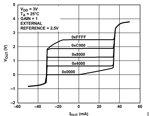
Figure 27. Source and Sink Capability at V_{DD} = 3 V
