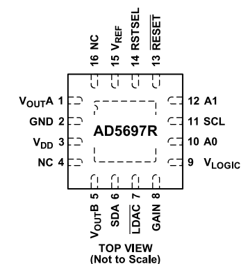
Figure 3. 16-Lead LFCSP Pin Configuration
