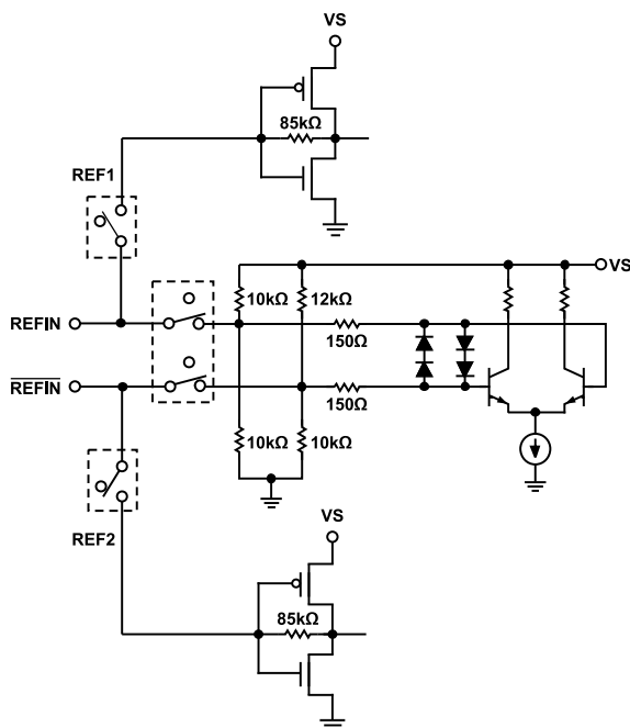
Figure 43. REF \overline{\text{IN}} Equivalent Circuit for Non-XTAL Mode
