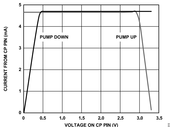
Figure 9. Charge Pump Characteristics at C_P = 3.3 V
