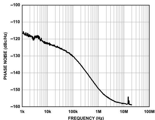
Figure 30. Phase Noise (Absolute) Clock Generation; Internal VCO at 2.212 GHz; PFD = 15.36 MHz; LBW = 66 kHz; LVPECL Output = 122.88 MHz
