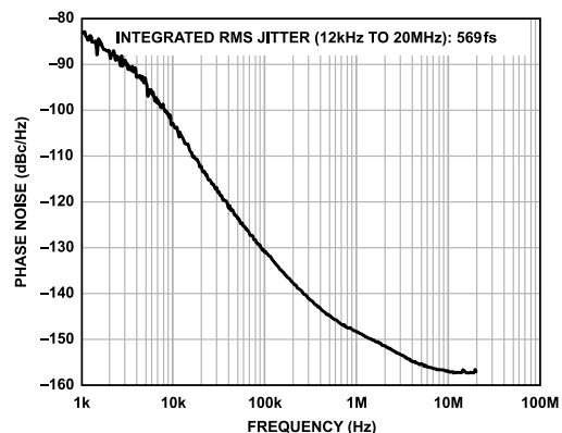
Figure 32. Phase Noise (Absolute) Clock Cleanup; Internal VCO at 2.177 GHz; PFD = 120 kHz; LBW = 2.18 kHz; LVPECL Output = 155.52 MHz
