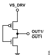
Figure 55. CMOS Equivalent Output Circuit
