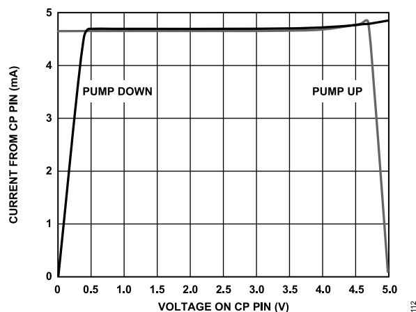
Figure 10. Charge Pump Characteristics at C_P = 5.0 V
