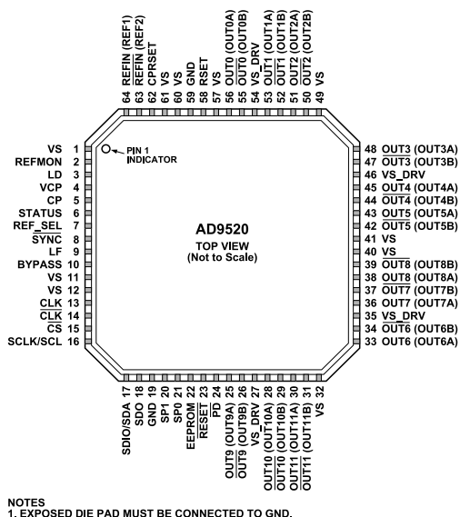
Figure 5. Pin Configuration
