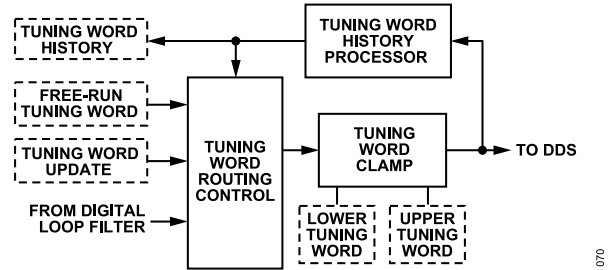
Figure 44. Tuning Word Processing
