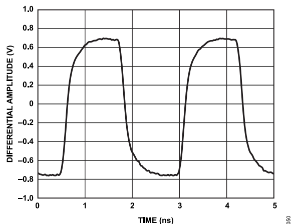
Figure 20. Output Waveform, LVPECL (400 MHz)
