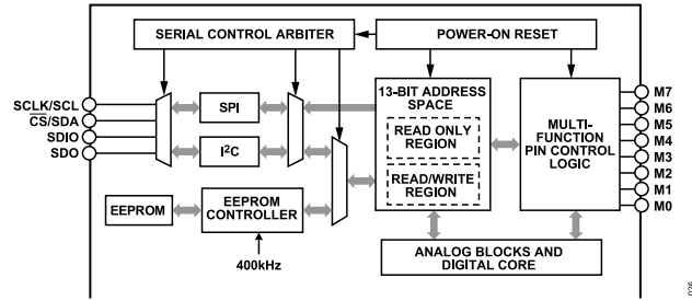
Figure 51. Serial Port Functional Diagram
