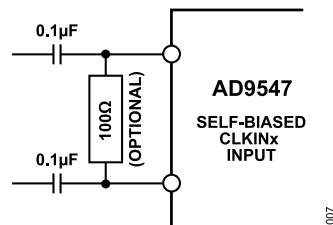
Figure 30. CLKINx Input
