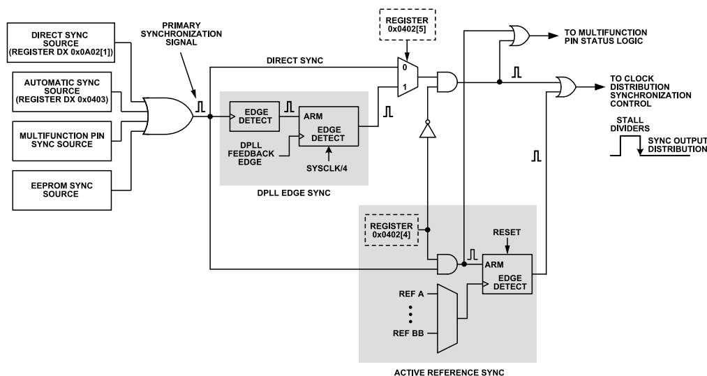
Figure 48. Output Synchronization Block Diagram
