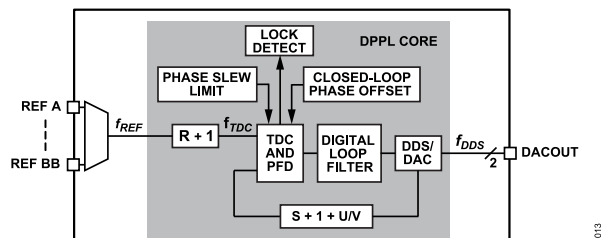
Figure 37. Digital PLL Core
