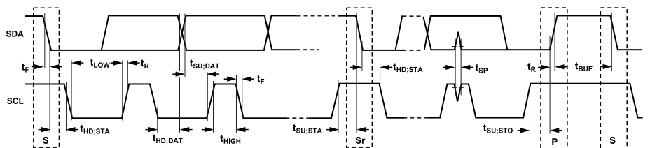
Figure 65. I 2 C Serial Port Timing
