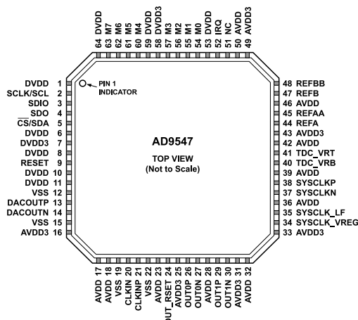
Figure 2. Pin Configuration
