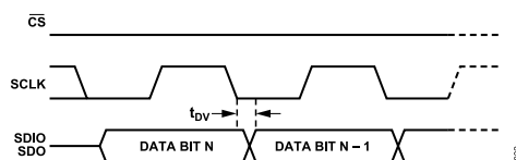
Figure 57. Serial Control Port Timing—Read
