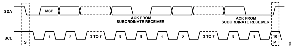
Figure 63. Data Transfer Process (Main Write Mode, 2-Byte Transfer Used for Illustration)
