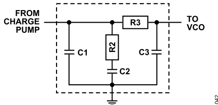
Figure 67. Third-Order Analog Loop Filter
