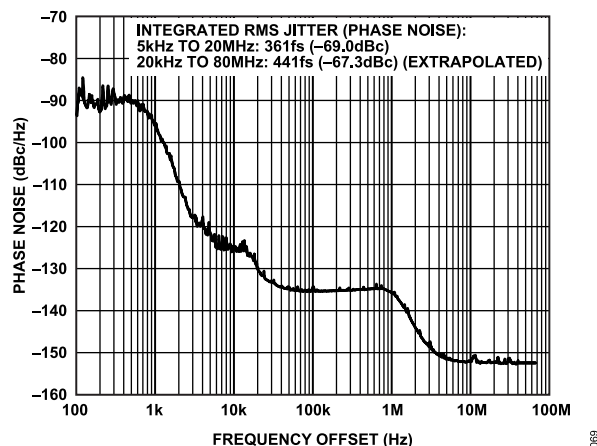
Figure 7. Absolute Phase Noise (Output Driver = LVPECL), f_{REF} = 19.44 MHz, f_0 = 155.52 MHz, LBW = 1 kHz, f_{SYSCLK} = 50 MHz, PLL On
