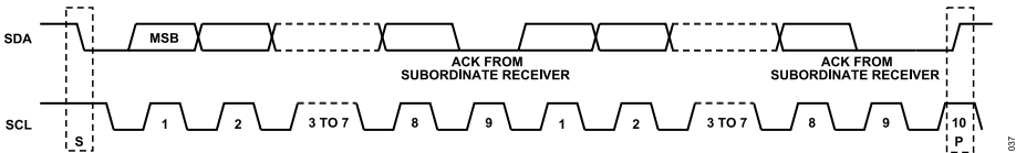
Figure 62. Acknowledge Bit
