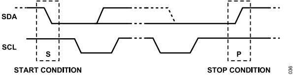
Figure 61. Start and Stop Condition
