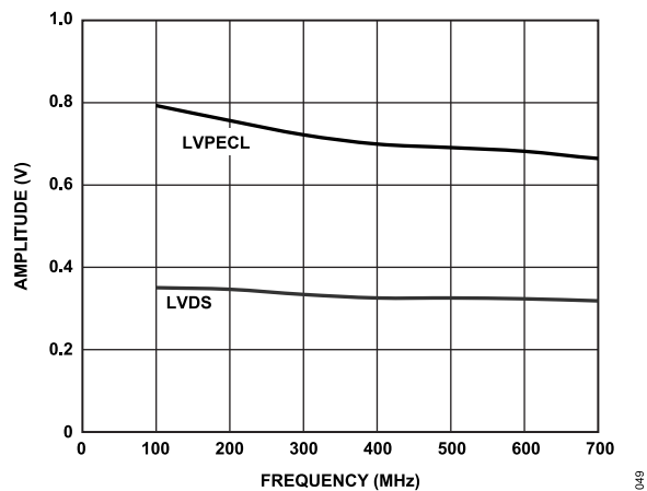
Figure 13. Amplitude vs. Toggle Rate, LVPECL and LVDS
