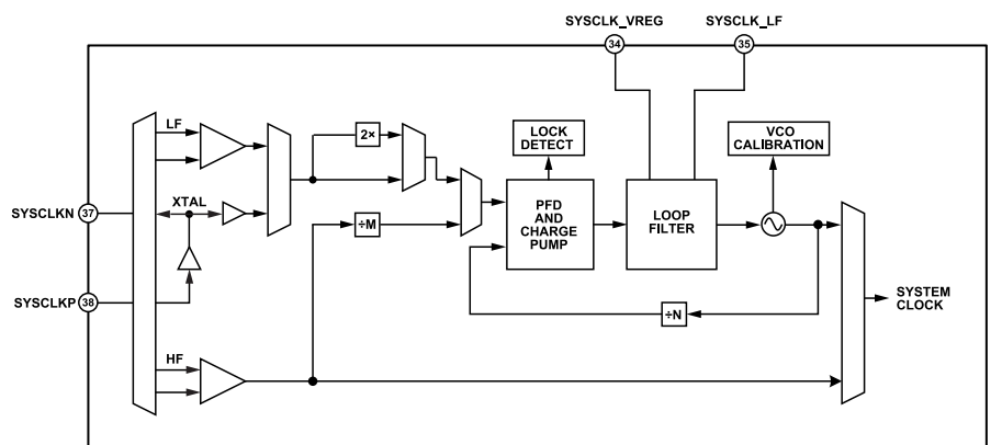
Figure 45. System Clock Block Diagram
