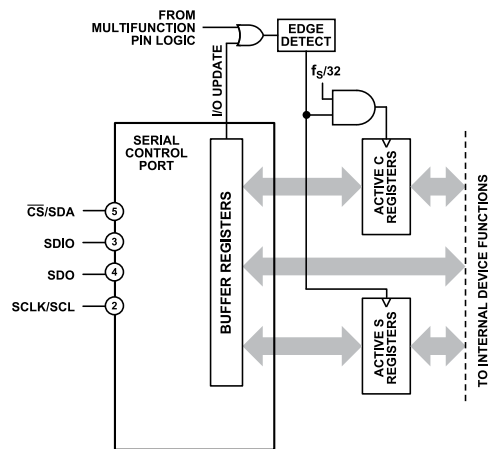
Figure 66. Buffered and Active Registers
