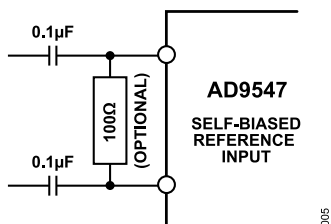
Figure 28. Reference Input
