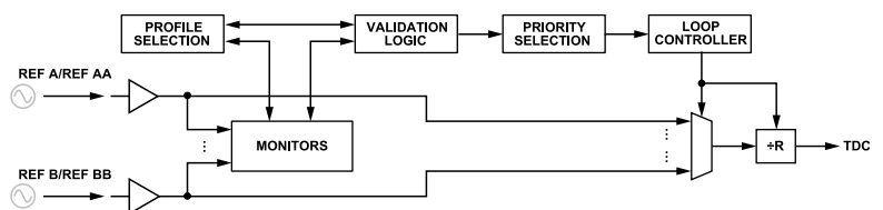
Figure 36. Reference Clock Block Diagram
