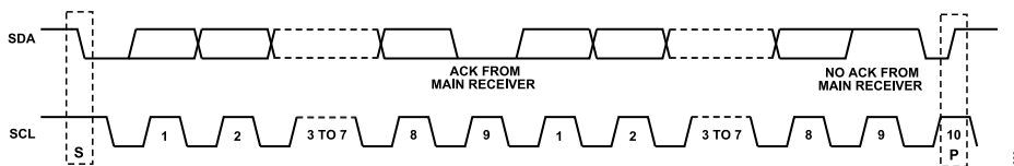
Figure 64. Data Transfer Process (Main Read Mode, 2-Byte Transfer Used for Illustration)
