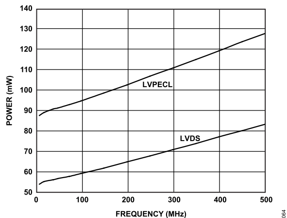
Figure 15. Power Consumption vs. Frequency, LVPECL and LVDS (Single Channel)
