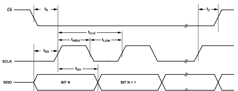
Figure 59. Serial Control Port Timing—Write
