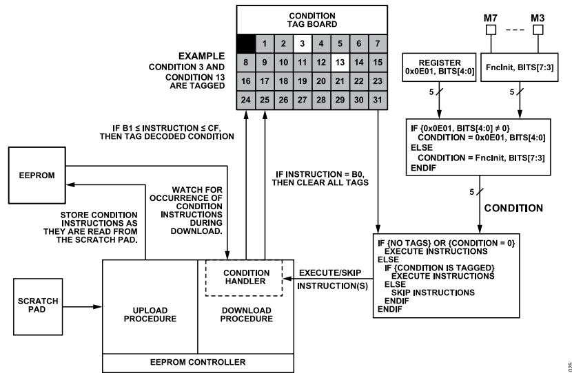
Figure 50. EEPROM Conditional Processing
