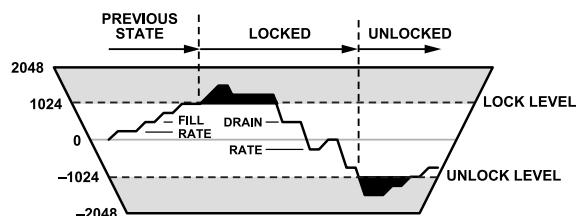
Figure 41. Phase Lock Detector Diagram
