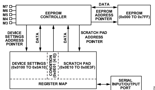
Figure 49. EEPROM Functional Diagram
