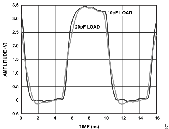
Figure 21. Output Waveform, 3.3 V CMOS (100 MHz, Strong Mode)
