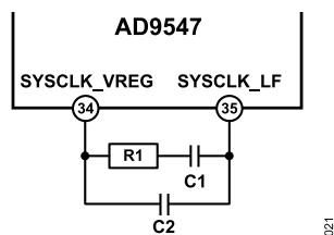
Figure 46. External Loop Filter Schematic
