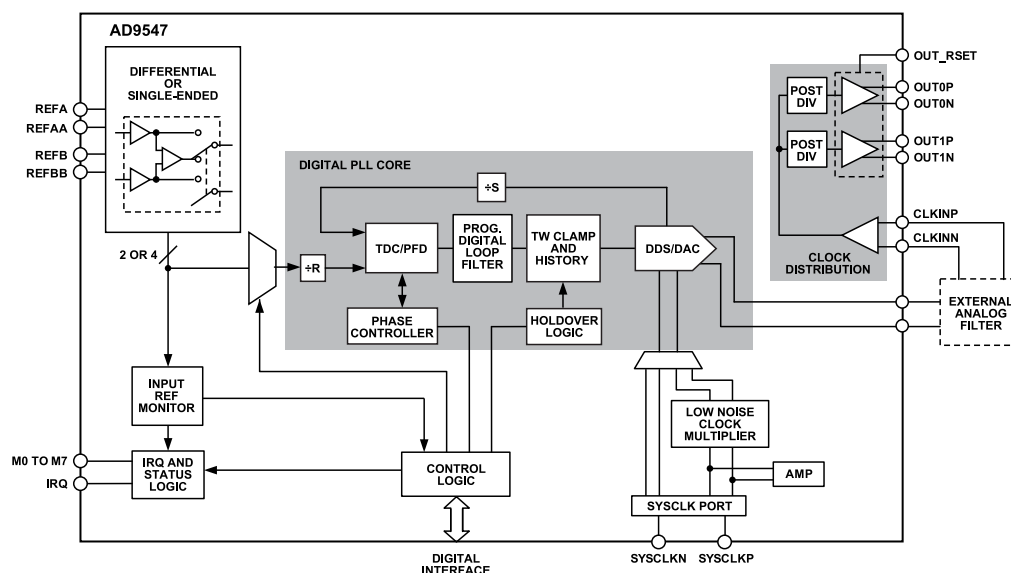
Figure 33. Detailed Block Diagram
