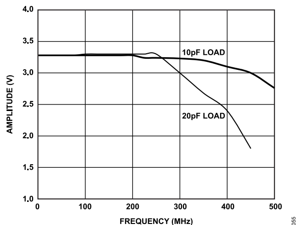
Figure 14. Amplitude vs. Toggle Rate, 3.3 V CMOS (Strong Mode)
