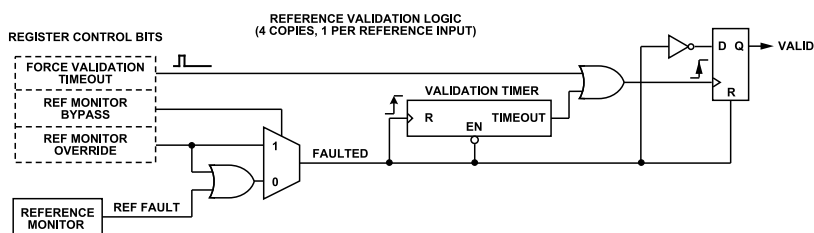
Figure 34. Reference Validation Override
