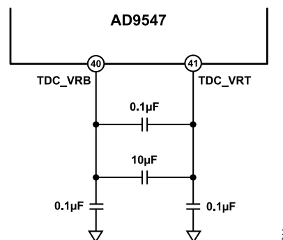
Figure 38. TDC Pin Connections
