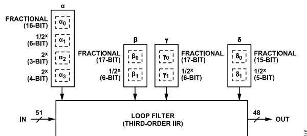
Figure 40. Third-Order Digital IIR Loop Filter
