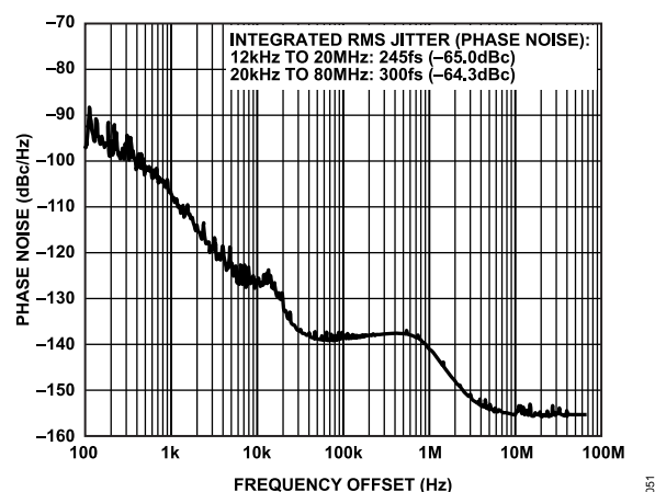
Figure 8. Absolute Phase Noise (Output Driver = LVPECL), f_{REF} = 19.44 MHz, f_0 = 155.52 MHz, LBW = 1 kHz, f_{SYSCLK} = 50 MHz (Crystal), PLL On with 2x Frequency Multiplier, I_{CP} = 375 \mu A, LF = External (350 kHz)
