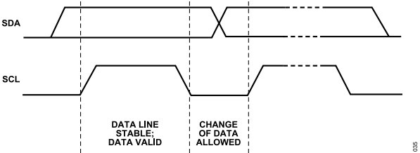
Figure 60. Valid Bit Transfer
