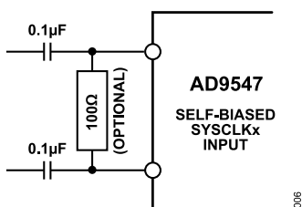
Figure 29. SYSCLKx Input
