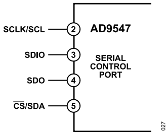
Figure 52. Serial Control Port
