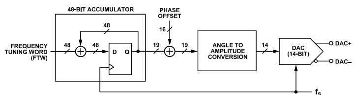
Figure 42. DDS Block Diagram
