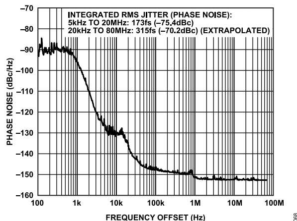
Figure 3. Absolute Phase Noise (Output Driver = LVPECL), f_{REF} = 19.44 MHz, f_O = 155.52 MHz, LBW = 1 kHz, f_{SYSCLK} = 1 GHz, PLL Off
