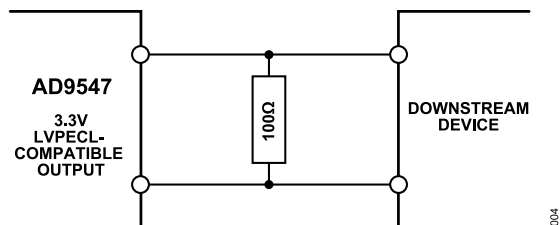
Figure 27. DC-Coupled LVDS or LVPECL Output Driver
