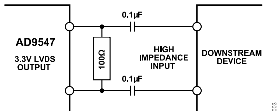
Figure 26. AC-Coupled LVDS or LVPECL Output Driver
