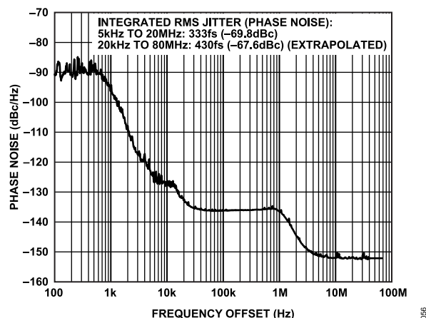
Figure 4. Absolute Phase Noise (Output Driver = LVPECL), f_{REF} = 19.44 MHz, f_O = 155.52 MHz, LBW = 1 kHz, f_{SYSCLK} = 50 MHz (Crystal), PLL On
