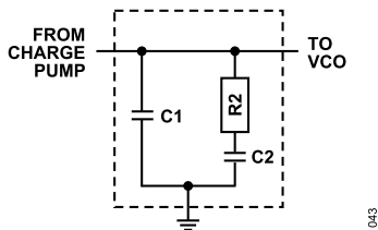
Figure 68. Second-Order Analog Loop Filter
