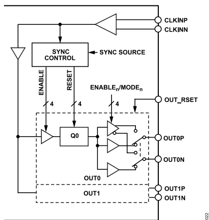
Figure 47. Clock Distribution
