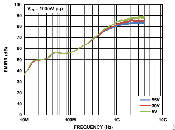
Figure 79. EMIRR vs. Frequency
