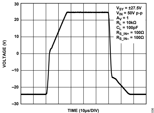
Figure 40. Large Signal Transient Response, V_{SY} = \pm 27.5 V
