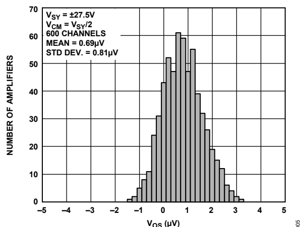
Figure 10. Input Offset Voltage Distribution, V_{SV} = \pm 27.5\text{ V}
