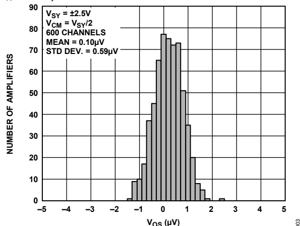
Figure 6. Input Offset Voltage Distribution, V_{SV} = \pm 2.5\text{ V}
