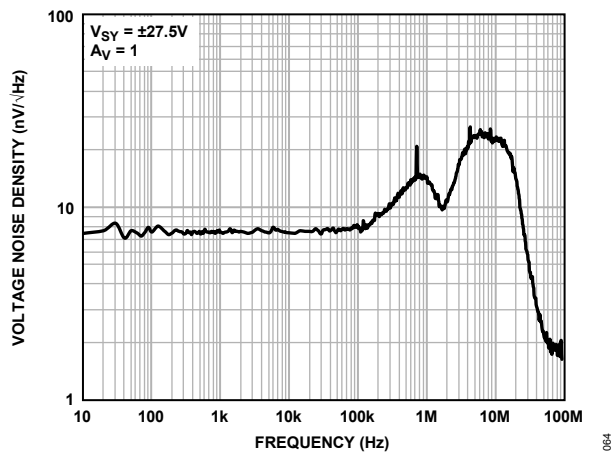
Figure 64. Voltage Noise Density vs. Frequency, V_{SV} = \pm 27.5\text{ V}
