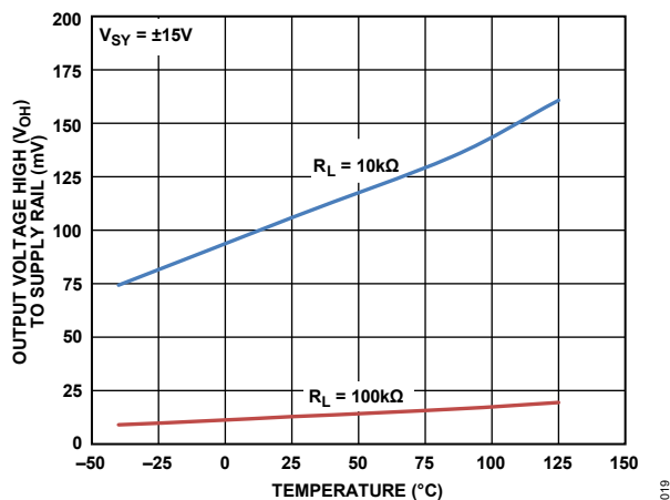
Figure 26. Output Voltage High ( V_{OH} ) to Supply Rail vs. Temperature, V_{SY} = \pm 15\text{ V}
