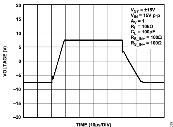
Figure 38. Large Signal Transient Response, V_{SY} = \pm 15 V
