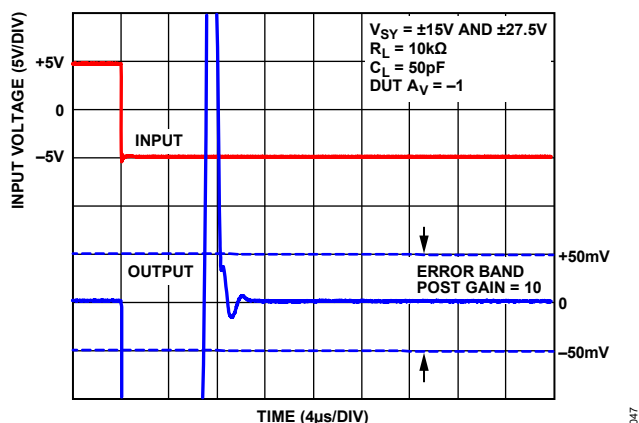
Figure 68. Negative Settling Time to 0.1%, V_{SY} = \pm 15V and \pm 27.5V
