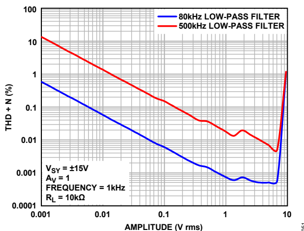
Figure 50. THD + N vs. Amplitude, V_{SY} = \pm 15\text{ V}
