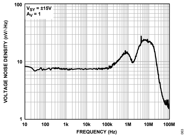
Figure 62. Voltage Noise Density vs. Frequency, V_{SV} = \pm 15\text{ V}
