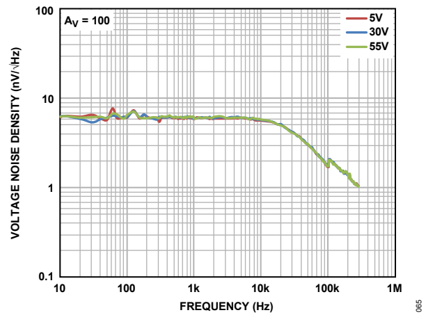
Figure 61. Voltage Noise Density vs. Frequency, V_{SV} = 5\text{ V}, 30\text{ V}, 55\text{ V}
