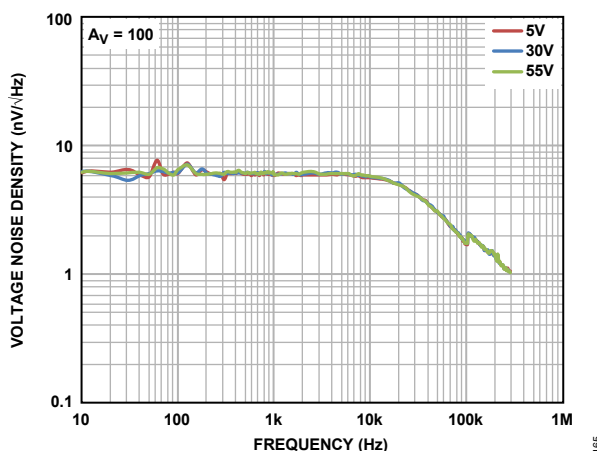
Figure 1. Voltage Noise Density vs. Frequency, V_{SV} = 5\text{ V} , 30 V, 55 V
