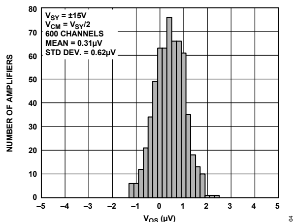
Figure 8. Input Offset Voltage Distribution, V_{SV} = \pm 15\text{ V}
