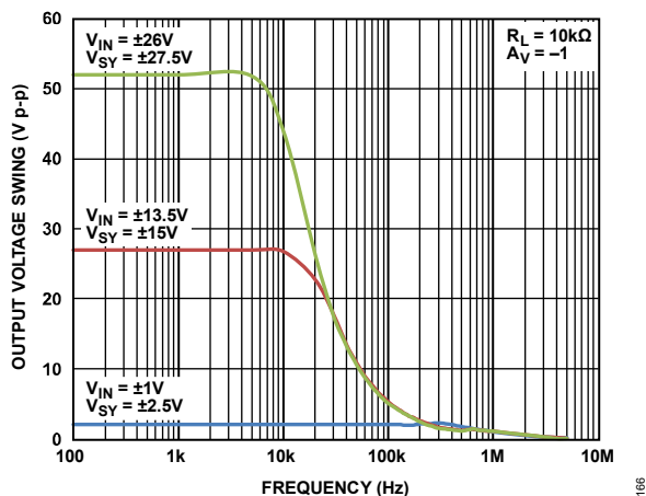
Figure 70. Output Voltage Swing vs. Frequency
