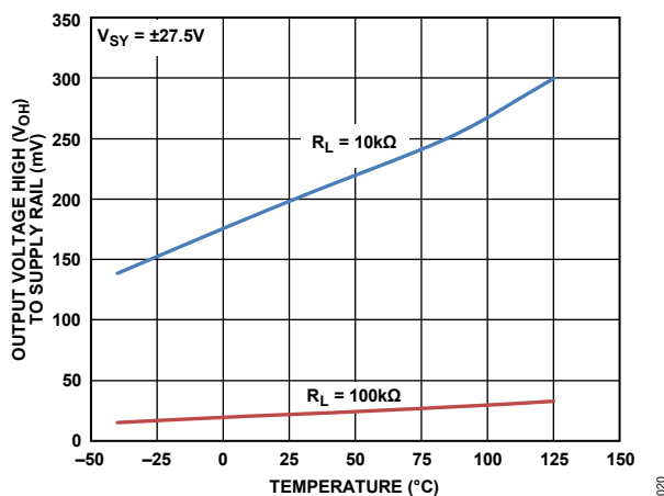
Figure 28. Output Voltage High ( V_{OH} ) to Supply Rail vs. Temperature, V_{SY} = \pm 27.5\text{ V}
