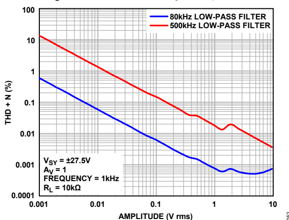
Figure 52. THD + N vs. Amplitude, V_{SY} = \pm 27.5\text{ V}
