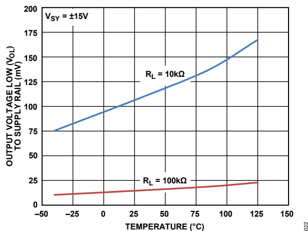
Figure 27. Output Voltage Low ( V_{OL} ) to Supply Rail vs. Temperature, V_{SY} = \pm 15\text{ V}
