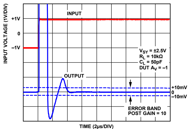
Figure 67. Positive Settling Time to 0.1%, V_{SY} = \pm 2.5V
