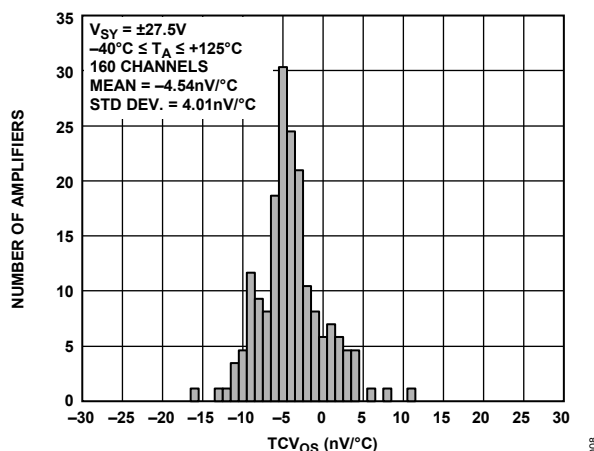
Figure 11. Input Offset Voltage Drift Distribution, V_{SV} = \pm 27.5\text{ V}
