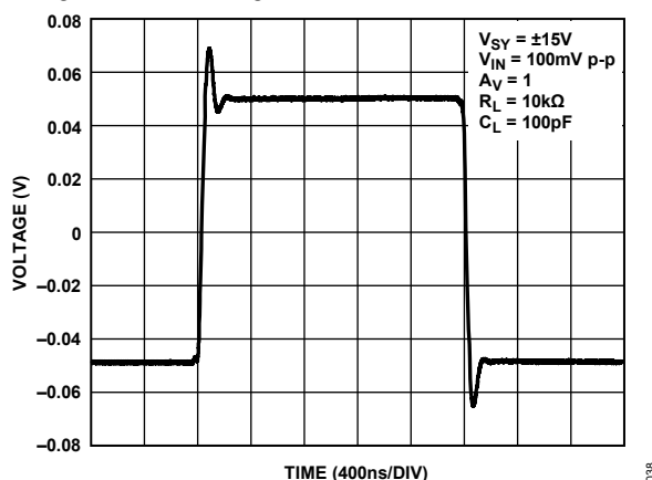
Figure 39. Small Signal Transient Response, V_{SY} = \pm 15 V
