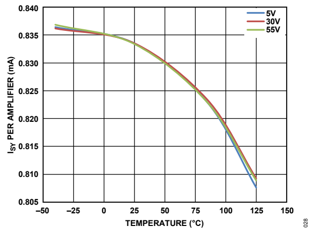
Figure 33. Supply Current ( I_{SY} ) per Amplifier vs. Temperature, V_{SY} = 5V, 30V, 55V
