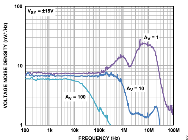
Figure 76. Voltage Noise Density with Various Gains
