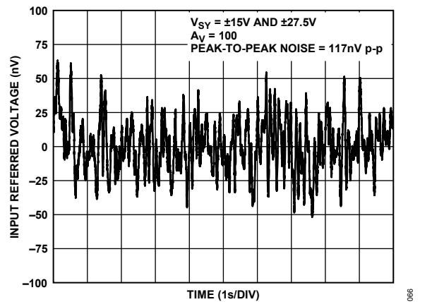
Figure 63. 0.1 Hz to 10 Hz Noise
