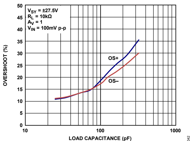
Figure 46. Small Signal Overshoot vs. Load Capacitance, V_{SY} = \pm 27.5\text{ V}
