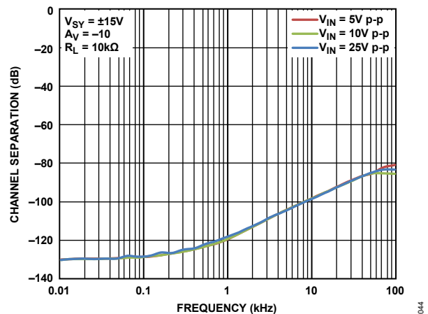
Figure 45. Channel Separation vs. Frequency, V_{SY} = \pm 15\text{ V}
