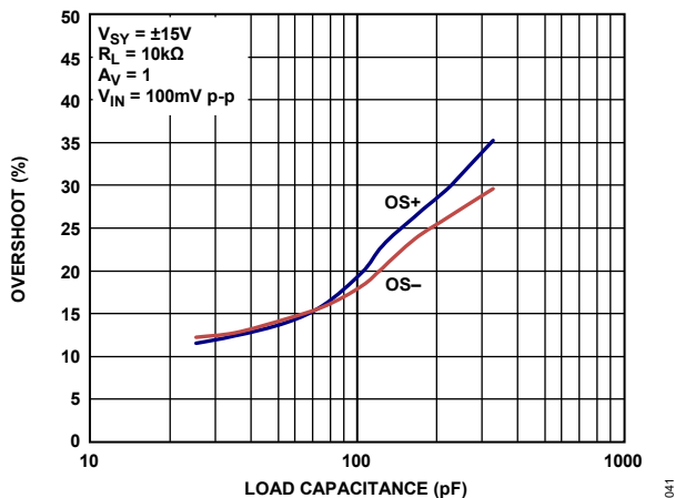
Figure 44. Small Signal Overshoot vs. Load Capacitance, V_{SY} = \pm 15\text{ V}
