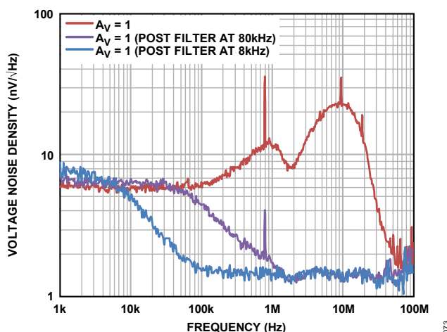
Figure 77. Voltage Noise Density with Post Filters
