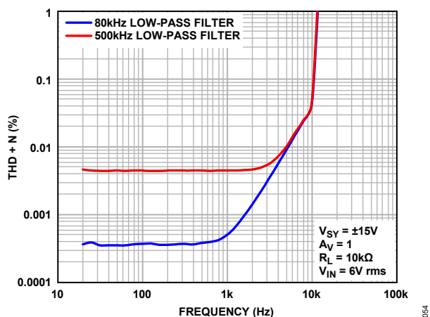
Figure 51. THD + N vs. Frequency, V_{SY} = \pm 15\text{ V}
