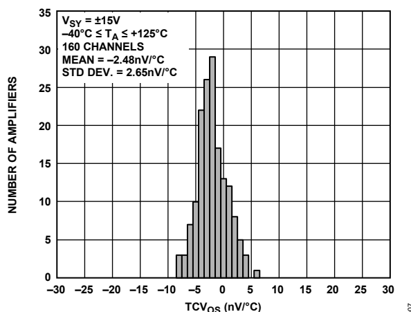
Figure 9. Input Offset Voltage Drift Distribution, V_{SV} = \pm 15\text{ V}
