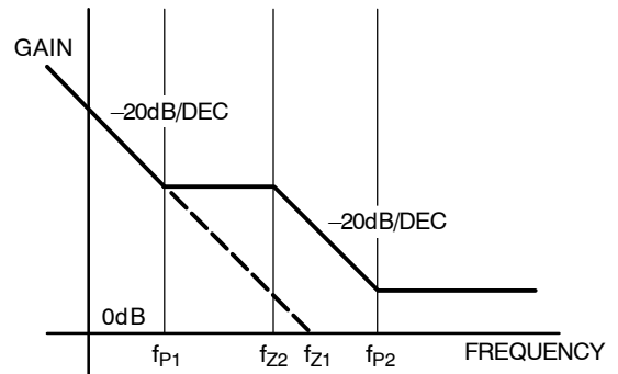
Figure 36. Poles and Zeros of Voltage Error Amplifier
