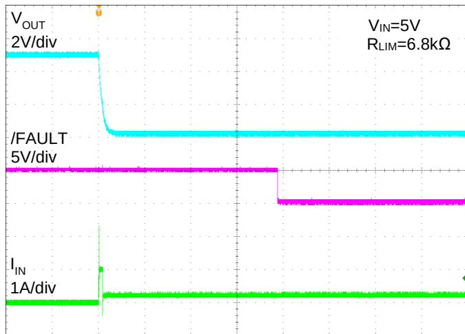
2ms/div No Load to 1 \Omega Transient Response
