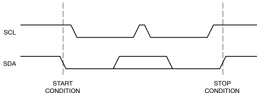
Figure 2. Start/Stop Timing
