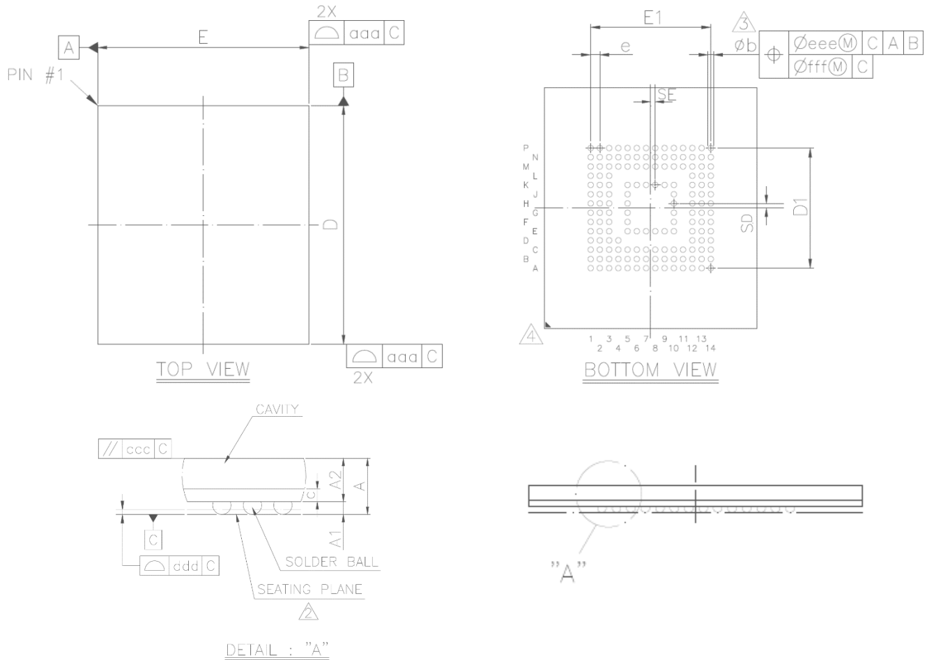
Figure 2 – Package Dimensions
