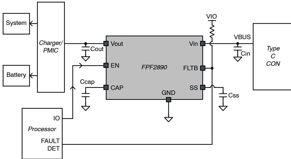
Figure 1. Typical Application
