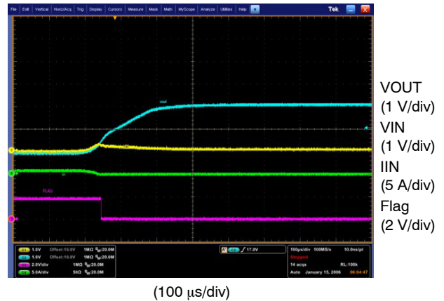
Figure 15. TRCB Behavior for Rout = 20 Ω (FLTb was configured active)
