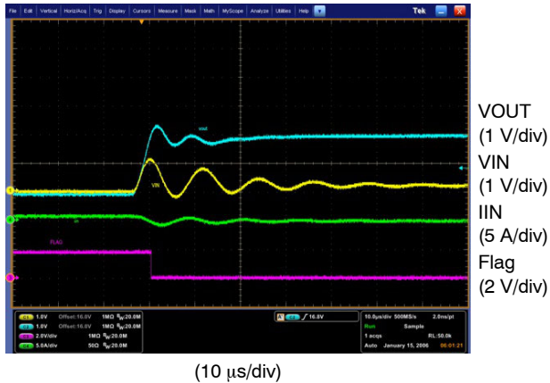
Figure 15. TRCB Behavior for Rout = 20 Ω (FLTb was configured active)
