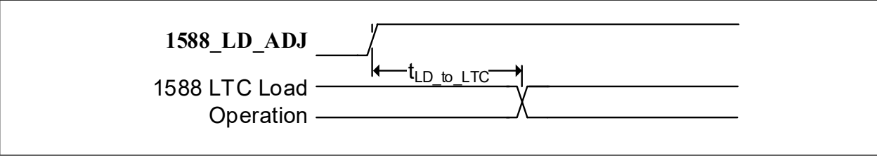
FIGURE 6-10: 1588_LD_ADJ TIMING
