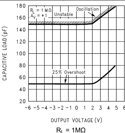
Figure 5-23. Stability vs Capacitive Load
