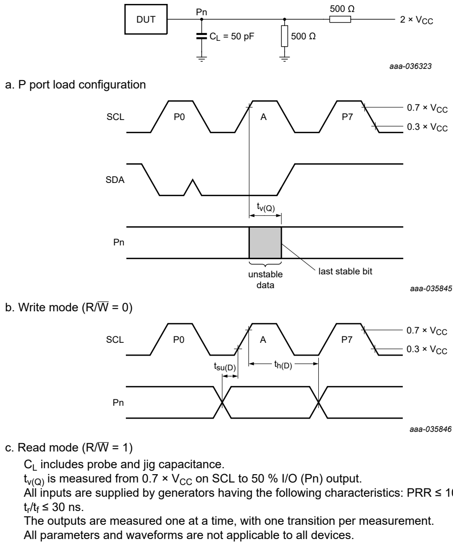
Fig. 27. P port load circuit and voltage waveforms
