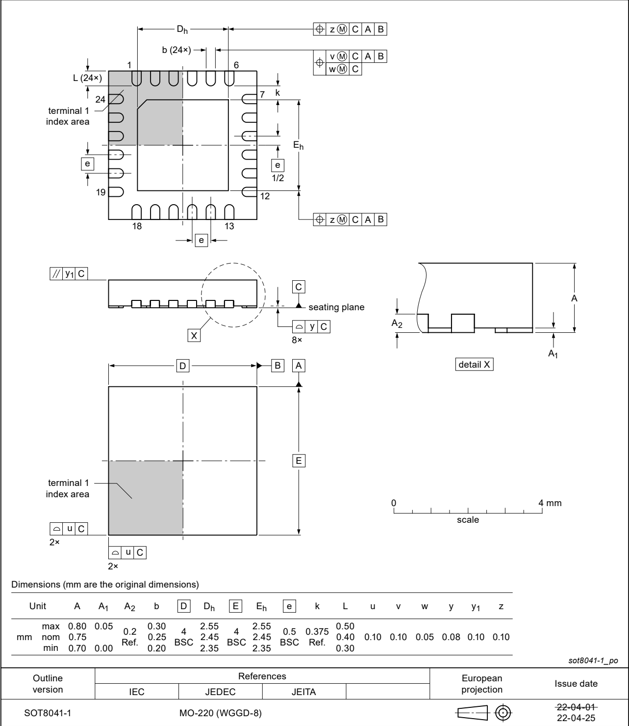
Fig. 29. Package outline SOT8041-1 (HWQFN24)
