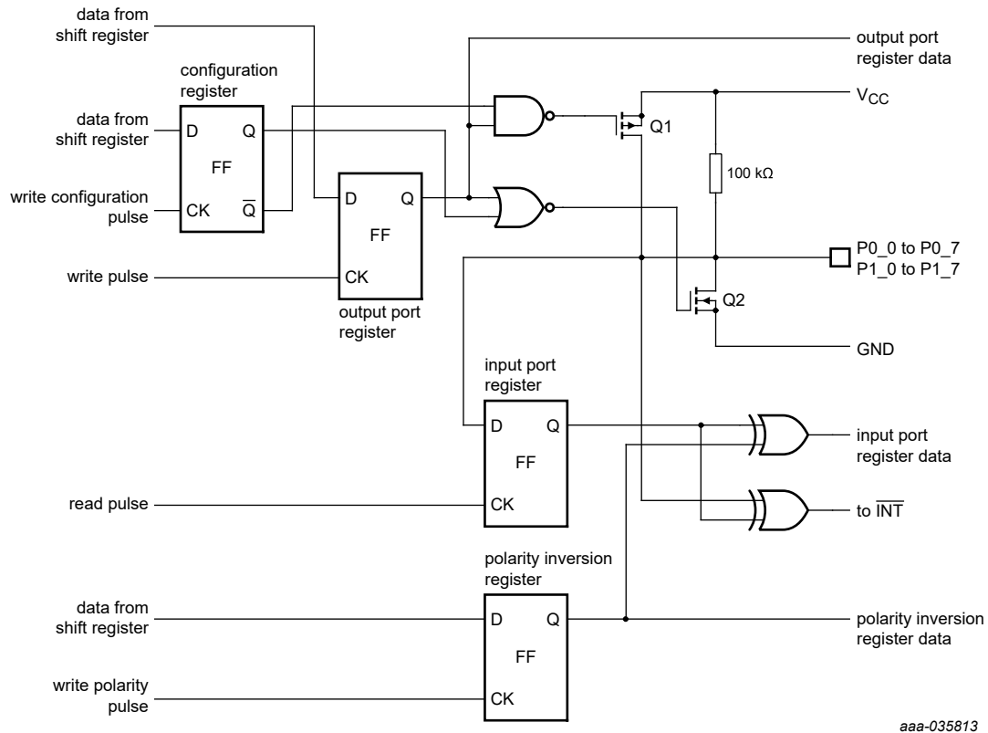
Fig. 4. Simplified schematic of the I/Os (P0_0 to P0_7, P1_0 to P1_7)
