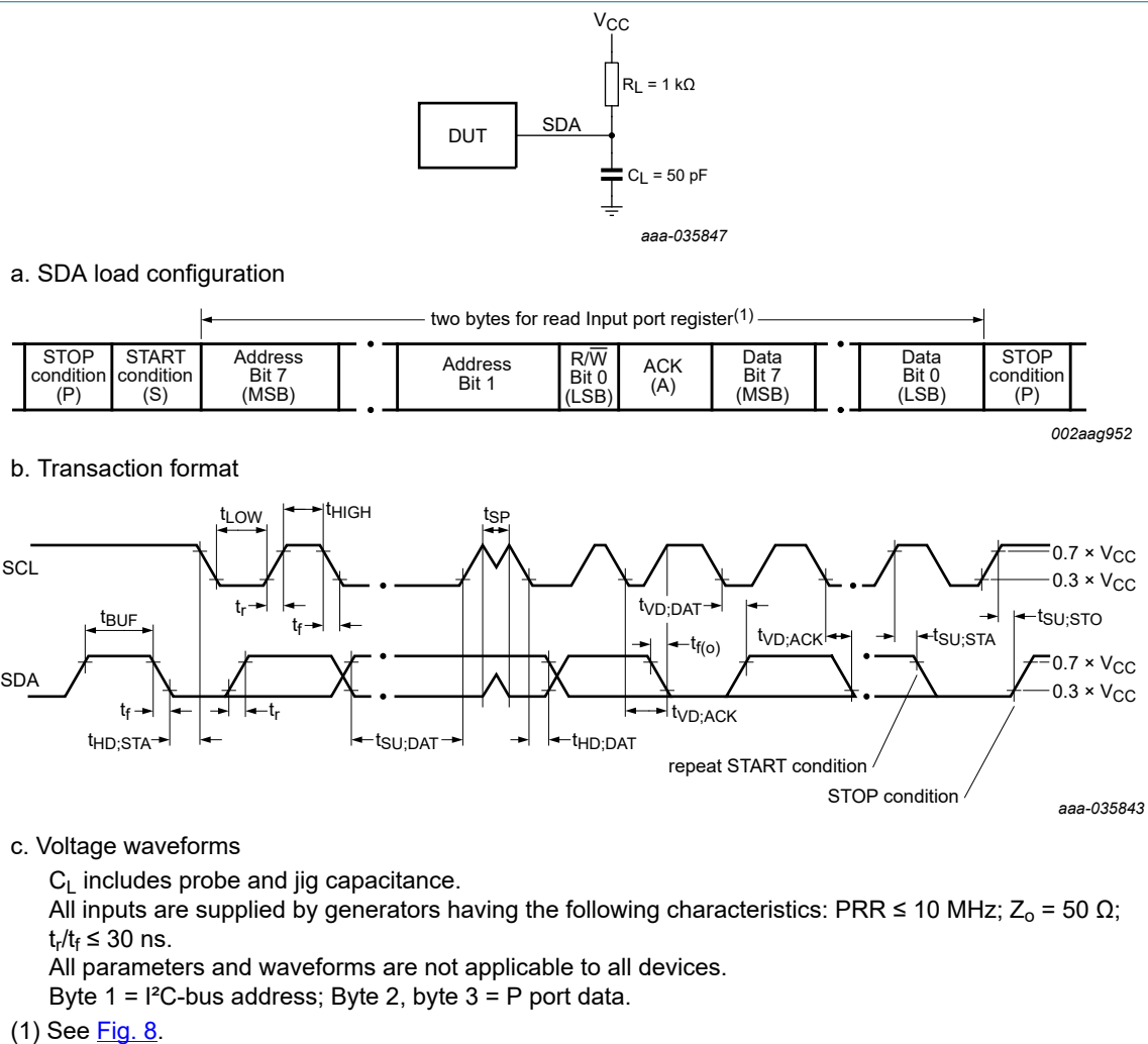
Fig. 25. I 2 C-bus interface load circuit and voltage waveforms
