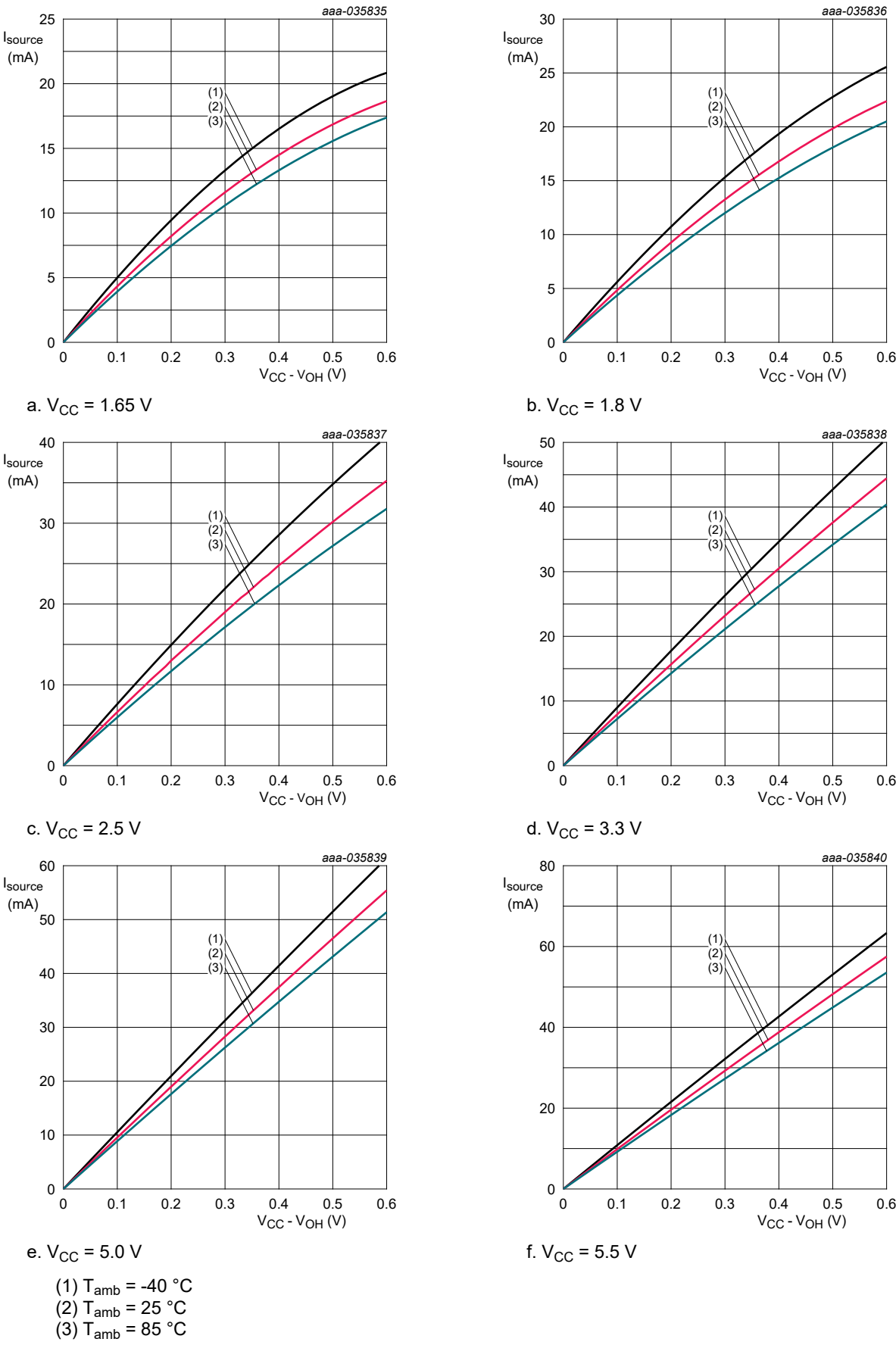
Fig. 23. I/O source current versus HIGH-level output voltage
