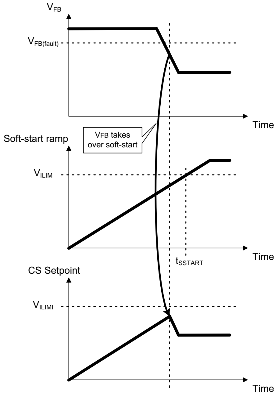
Figure 36. Soft-Start
