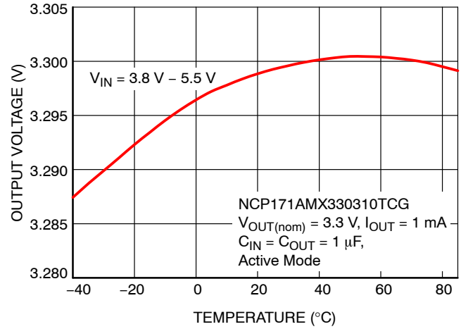
Figure 35. Output Voltage vs. Temperature in Active Mode
