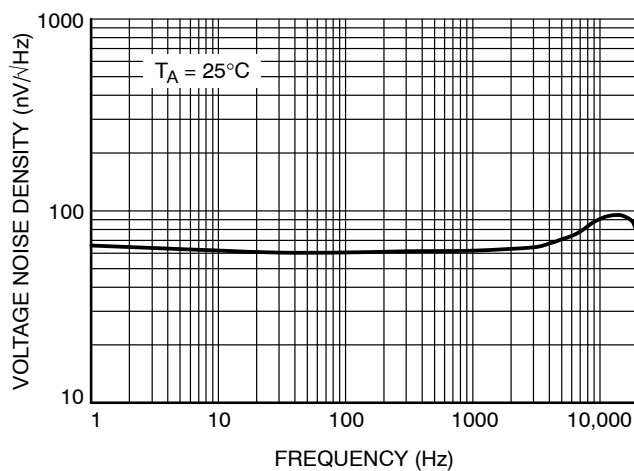
Figure 16. Voltage Noise Density vs. Frequency
