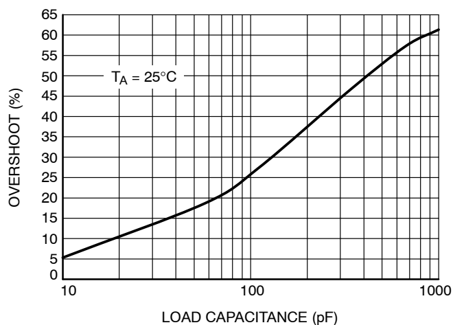
Figure 14. Small-Signal Overshoot vs. Load Capacitance
