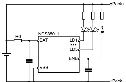
Figure 8. Poor Layout Practices: Stubs on Capacitors; Direct Path from Switches and LEDs to the IC; Multiple Connections to Pack+ and Pack-.
