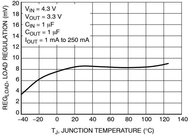
Figure 9. Load Regulation vs. Temperature – V OUT = 3.3 V
