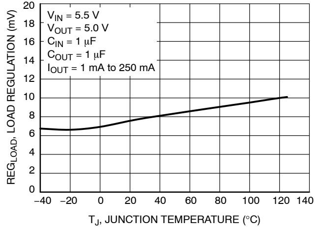
Figure 10. Load Regulation vs. Temperature – V OUT = 5.0 V
