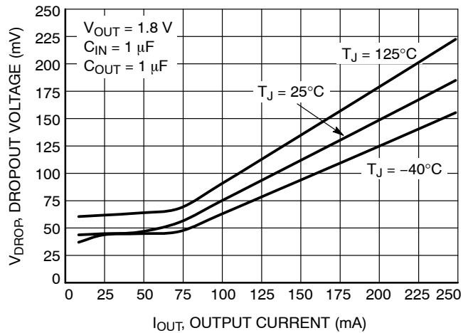
Figure 14. Dropout Voltage vs. Load Current – V OUT = 1.8 V – XDFN4 Package
