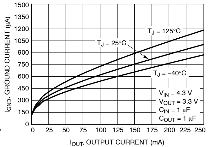
Figure 12. Ground Current vs. Load Current – V OUT = 3.3 V
