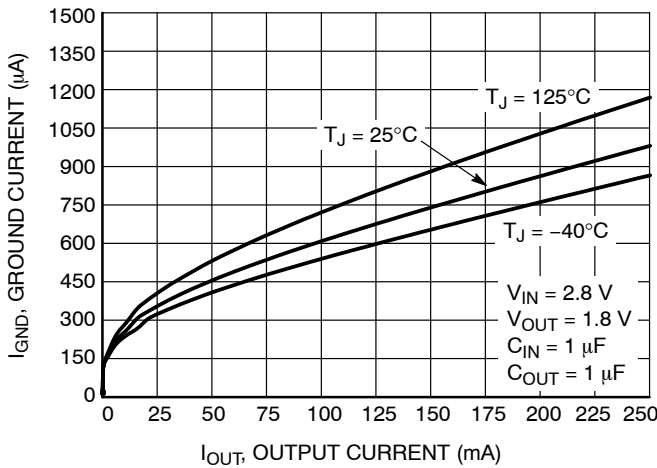
Figure 11. Ground Current vs. Load Current – V OUT = 1.8 V
