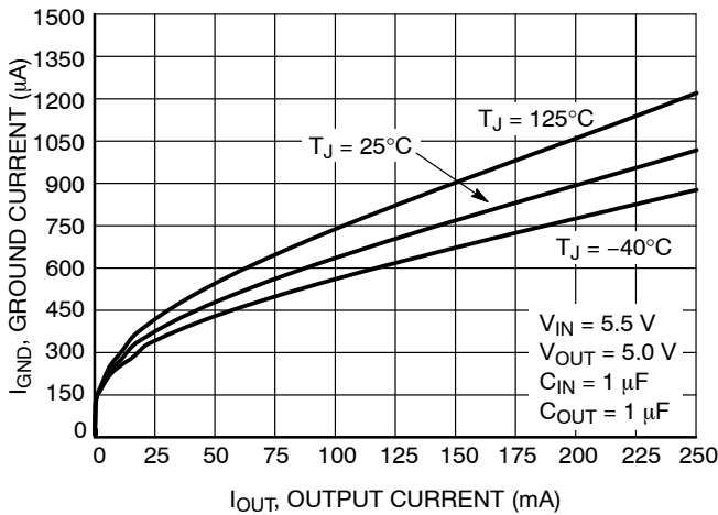
Figure 13. Ground Current vs. Load Current – V OUT = 5.0 V
