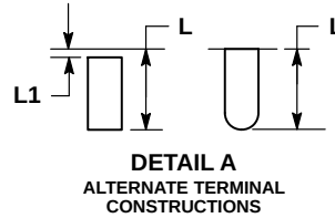
DFN6, 2x2.2, 0.65P CASE 506BA ISSUE A
