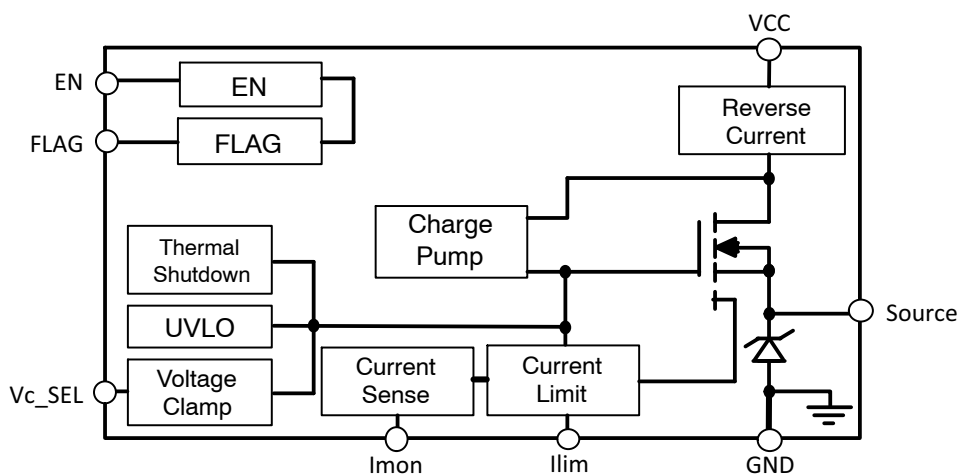
Figure 2. Block Diagram
