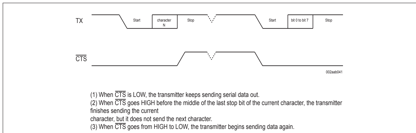
Figure 3. \overline{\text{CTS}} Functional Timing
