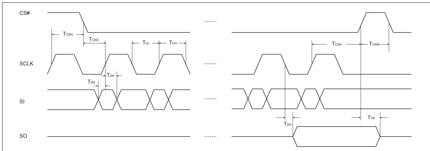
Figure 26. SPI-bus Timing
