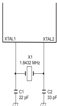
Figure 8. PCrystal Oscillator Circuit Reference
