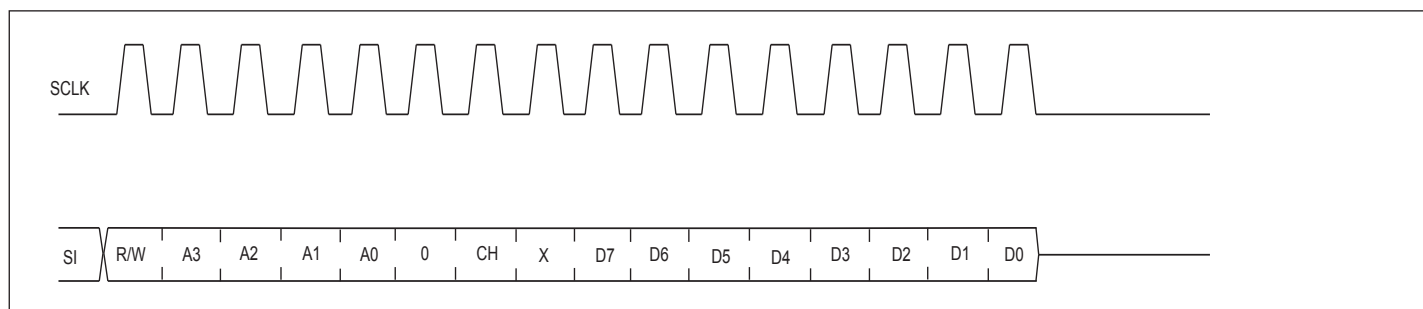
Figure 13. SPI Write
