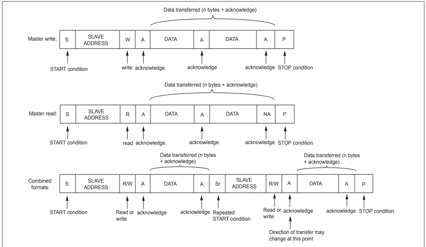
Figure 12. I²C Data Formats
