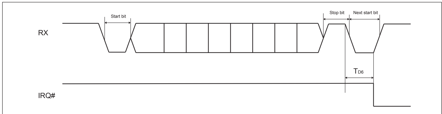
Figure 23. Receive Interrupt
