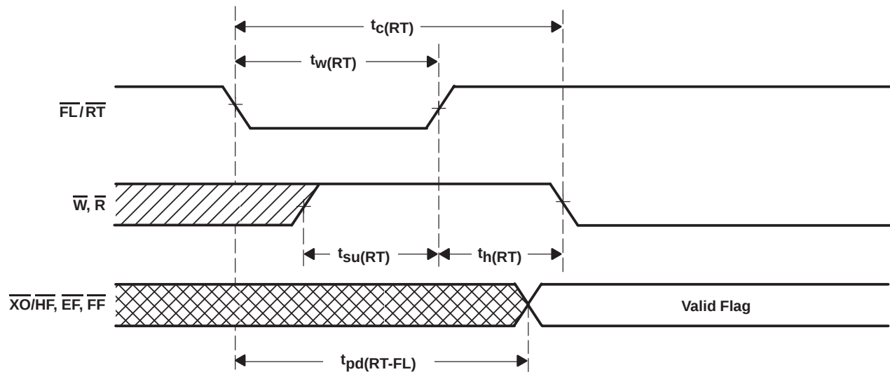
Figure 4. Retransmit Waveforms
