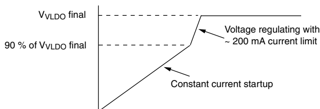
Figure 10 - LDO Start-Up
