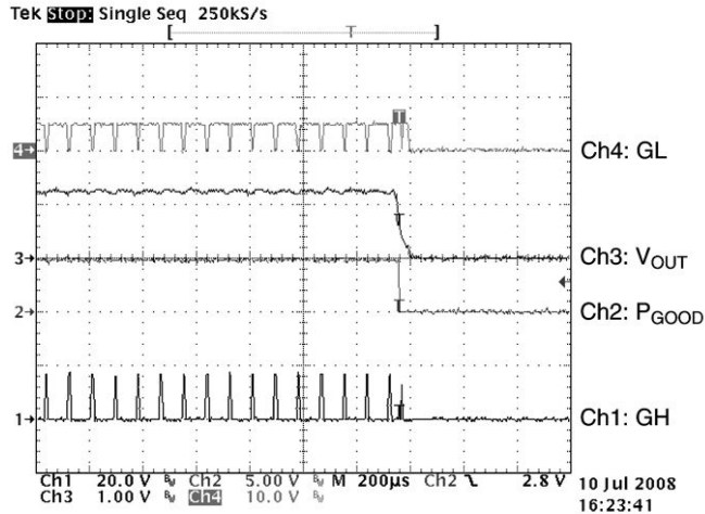
Over Current Protection: V IN = 12 V, V OUT = 1.2 V
