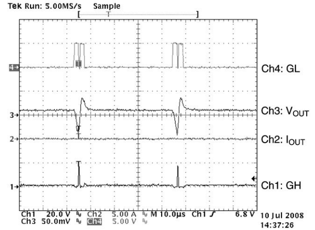
Ultra-Sonic Power-Save at I OUT = 0 A
