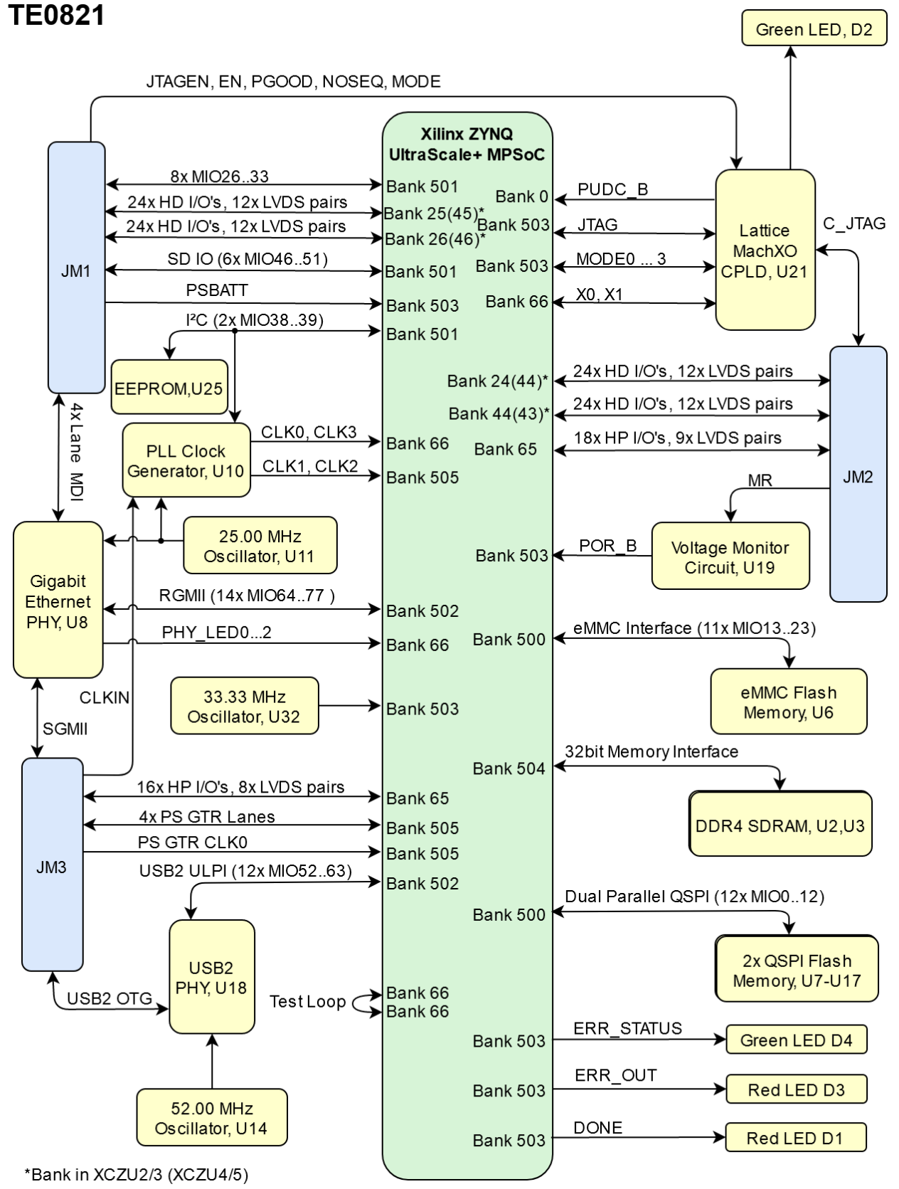
Figure 1: TE0821 block diagram
