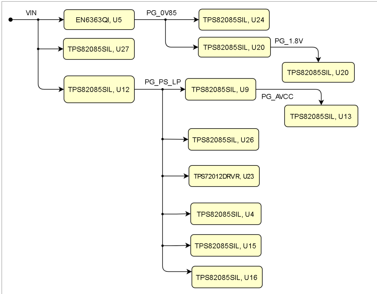
Figure 4: Power Sequence
