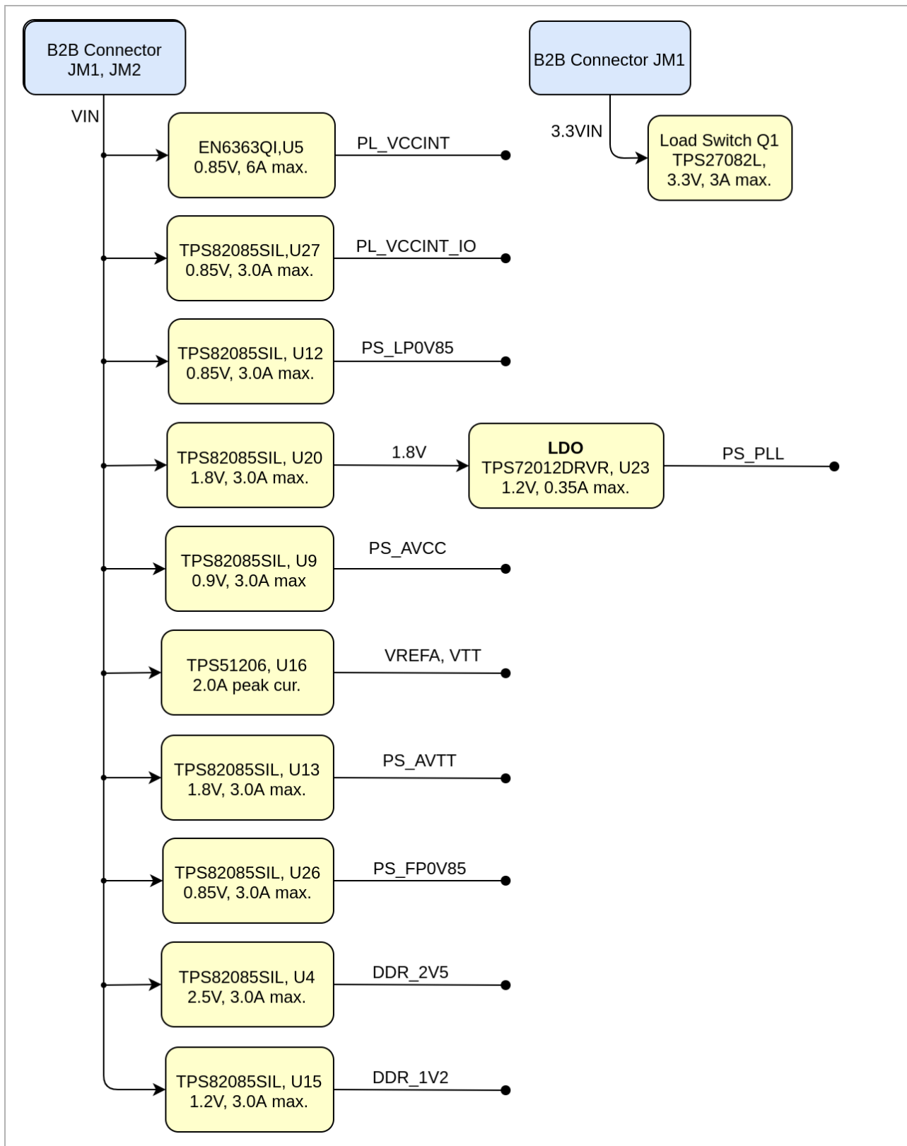
Figure 3: Power Distribution
