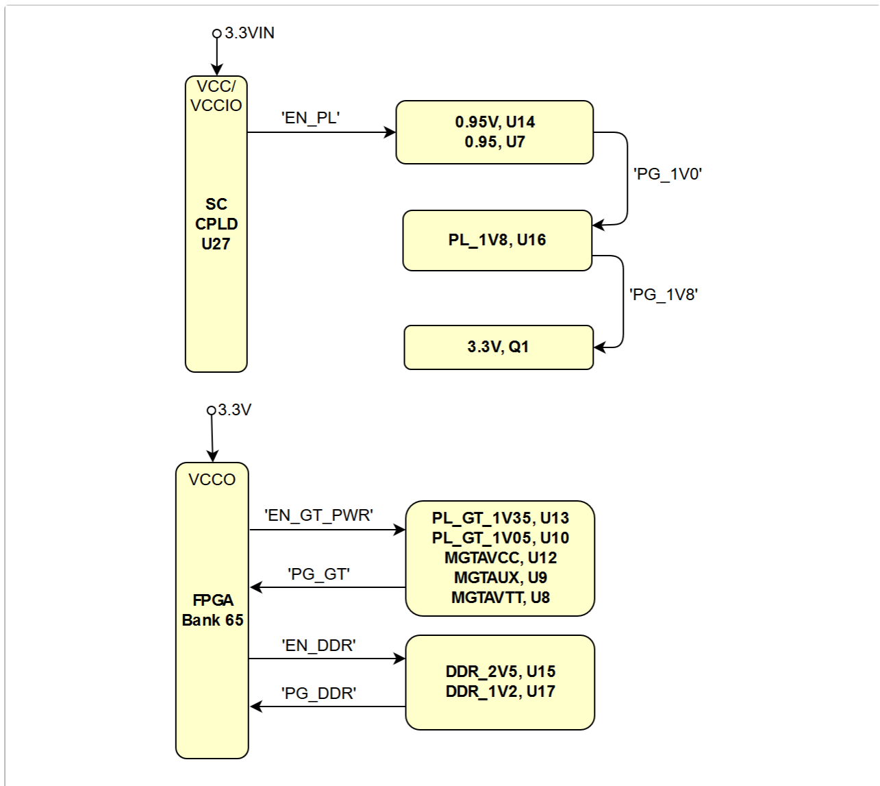
4 Figure 4: TE0841-02 Power-On Sequence Diagram
