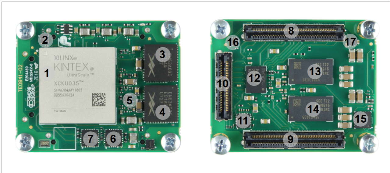
2 Figure 2: TE0841-02 main components
