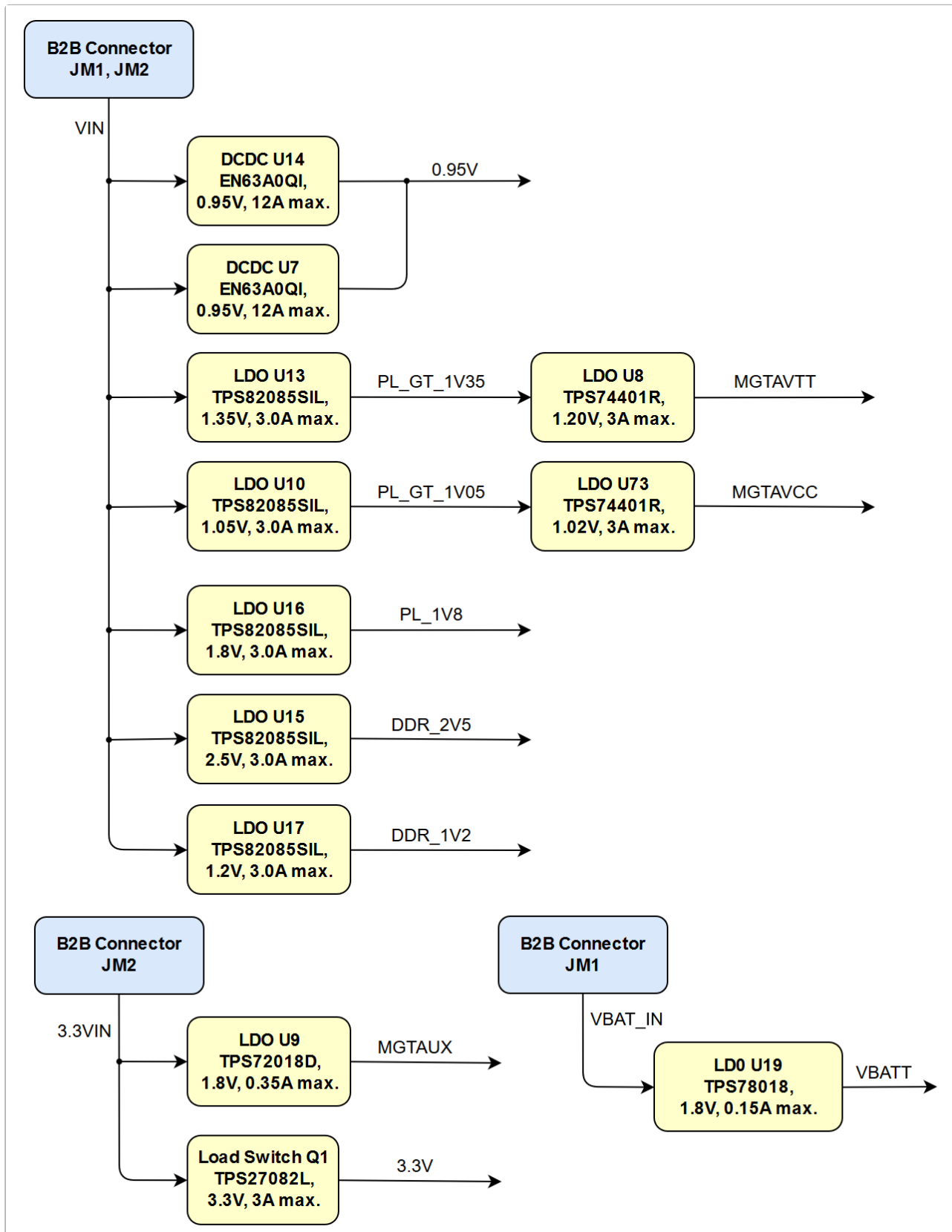
3 Figure 3: TE0841-02 Power Distribution Diagram
