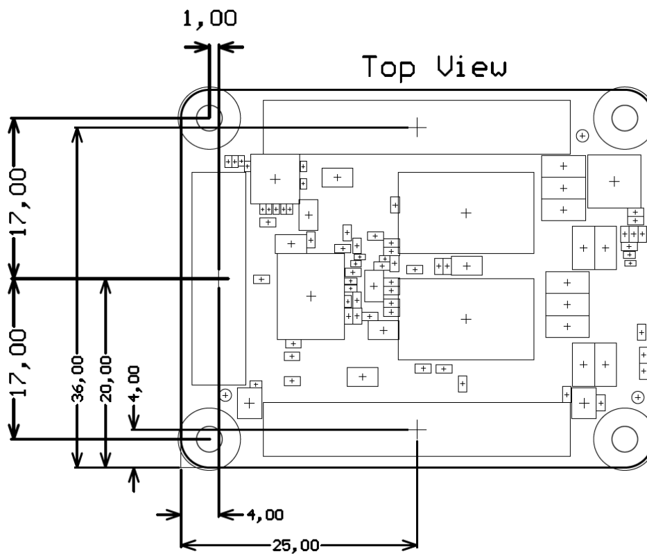
5 Figure 5: Module physical dimensions drawing
