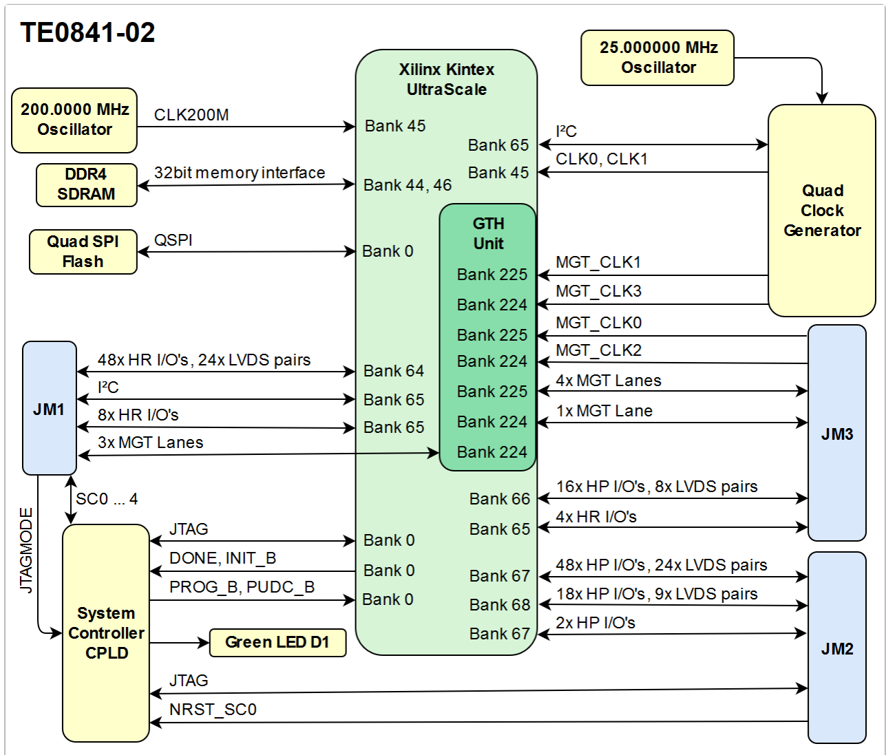
1 Figure 1: TE0841-02 block diagram
