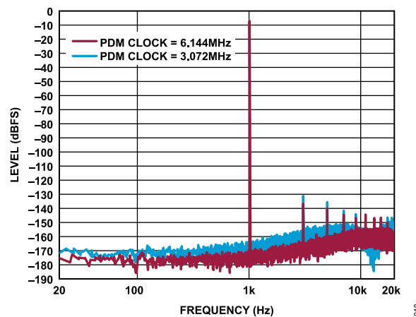
Figure 18. FFT, -7 dBFS, f_S = 48 kHz Throughout, Signal Path = SDATAI_x to FastDSP to PDM Output
