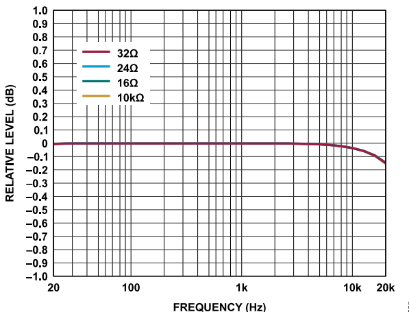
Figure 32. Relative Level vs. Frequency, f_s = 48 kHz, Signal Path = SDATAI_x to HPOUT/LOUT, 16 \Omega , 24 \Omega , 32 \Omega , or 10 k \Omega
