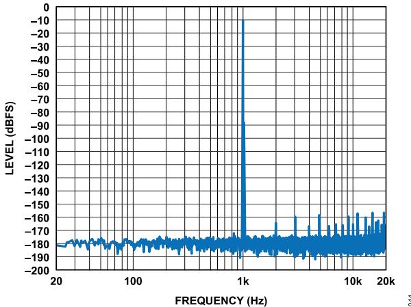
Figure 44. FFT, -10 \text{ dBFS} Input, \text{DMIC\_CLK\_RATE} = 6.144 \text{ MHz} , Signal Path = DMICxx to SDATAO_x
