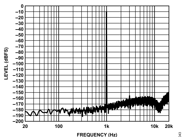
Figure 43. FFT, -10 \text{ dBFS} Input, \text{DMIC\_CLK\_RATE} = 3.072 \text{ MHz} , Signal Path = DMICxx to SDATAO_x
