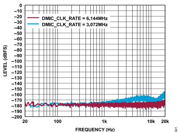
Figure 41. FFT, No Signal, \text{DMIC\_CLK\_RATE} = 3.072 \text{ MHz} and 6.144 \text{ MHz} , Signal Path = DMICxx to SDATAO_x
