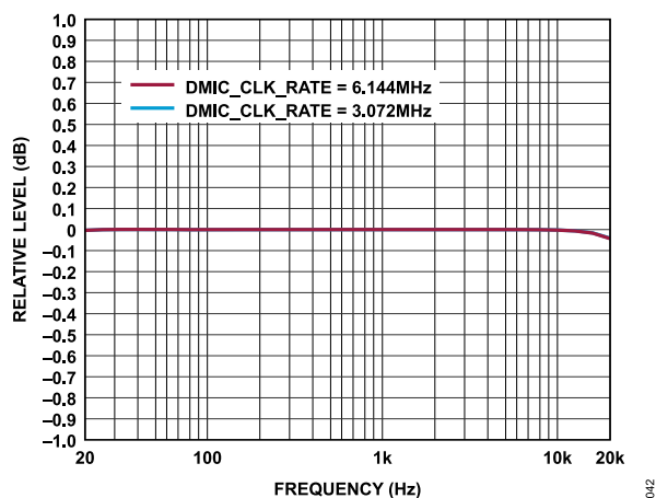
Figure 42. Relative Level vs. Frequency, \text{DMIC\_CLK\_RATE} = 3.072 \text{ MHz} and 6.144 \text{ MHz} , Signal Path = DMICxx to SDATAO_x, FCOMP = EN
