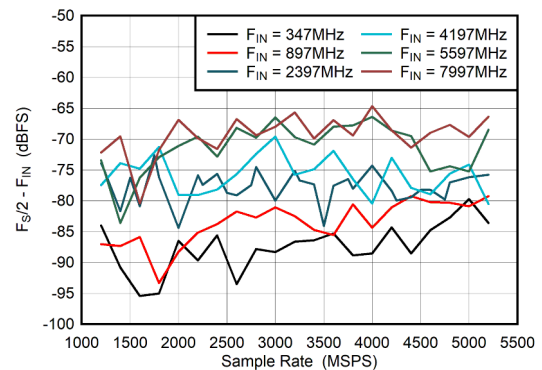
Figure 5-56. Dual Channel Mode: F_{\text{S}}/2 - F_{\text{IN}} vs Sample Rate
