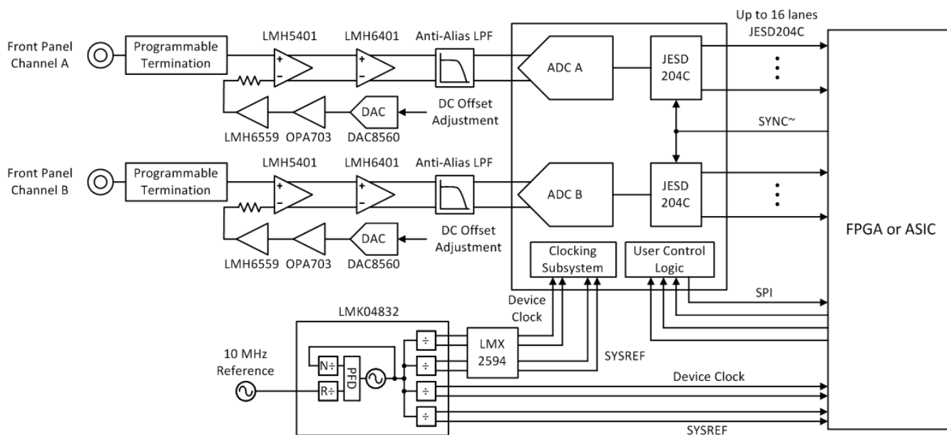
Figure 7-1. Typical Configuration for Reconfigurable Oscilloscope
