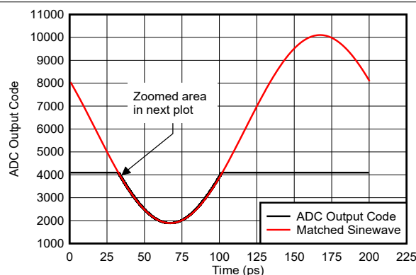
Figure 5-148. Sinewave Overdrive Recovery
