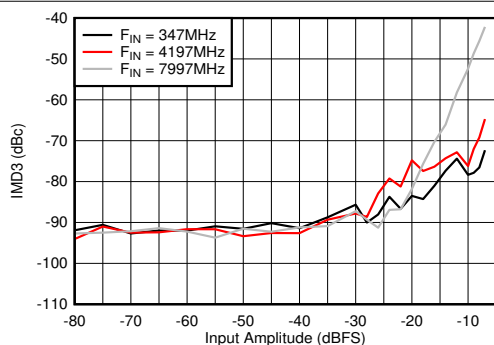
Figure 5-105. Dual Channel Mode: IMD3 vs Input Amplitude
