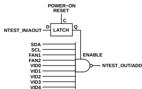
Figure 36. NAND Tree
