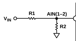
Figure 14. Scaling A_{IN(1-2)}
