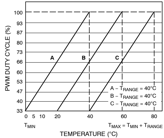
Figure 31. Effect of Increasing T_{\text{MIN}} Value on Control Loop
