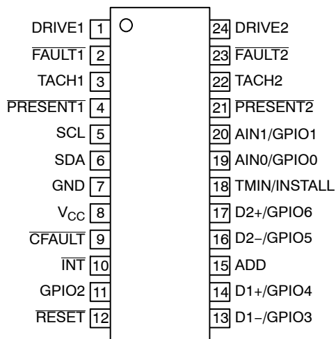
ADM1029 Top View (Not To Scale)
