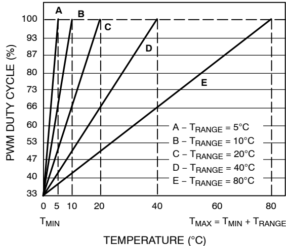
Figure 30. PWM Duty Cycle vs. Temperature Slopes ( T_{\text{RANGE}} )
