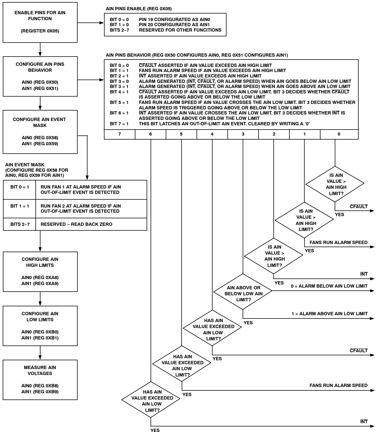
Figure 38. Configuring AIN0 and AIN1 Pins
