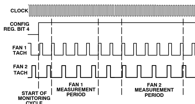
Figure 24. Fan Speed Measurement
