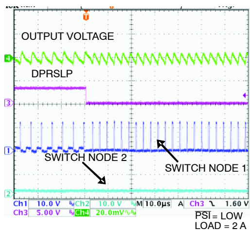
Figure 24. DPRSLP Transition
