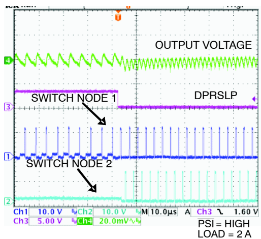
Figure 22. DPRSLP Transition
