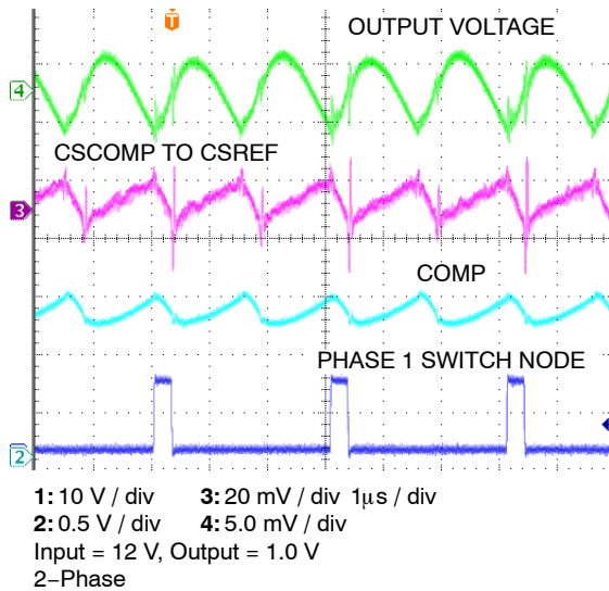
Figure 13. Switching Waveforms
