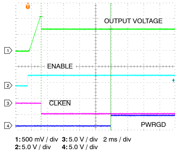
Figure 8. Startup Waveforms
