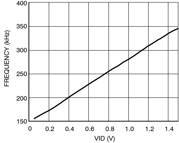
Figure 6. Master Clock vs. VID
