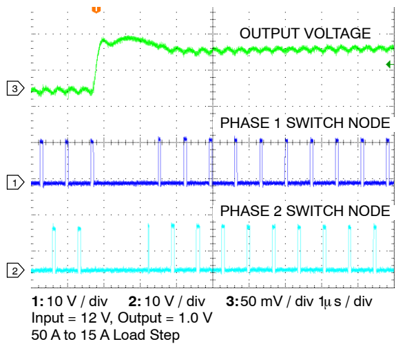
Figure 10. Load Transient with 2-Phases
