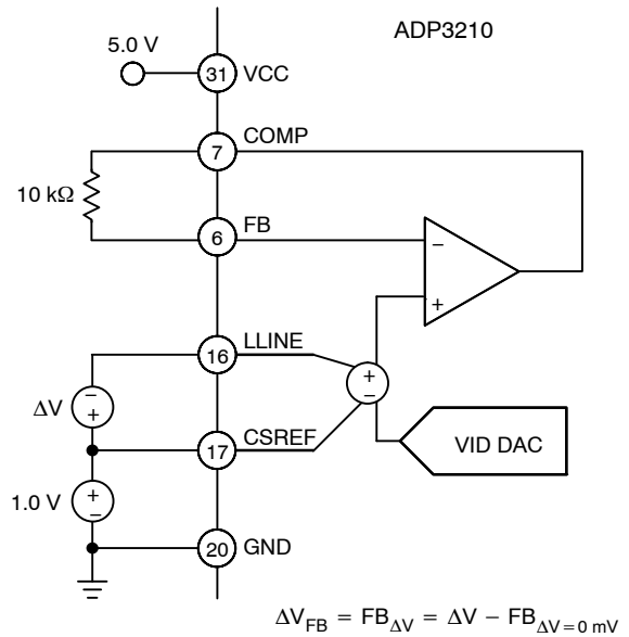
Figure 4. Positioning Accuracy
