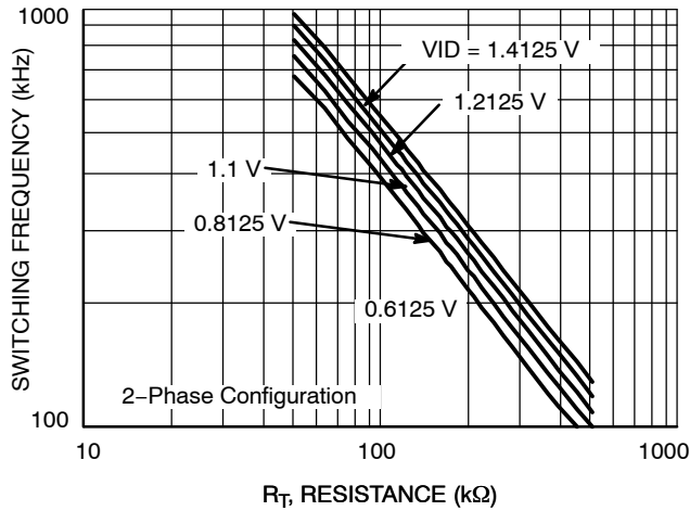
Figure 5. Master Clock Frequency vs. R_T
