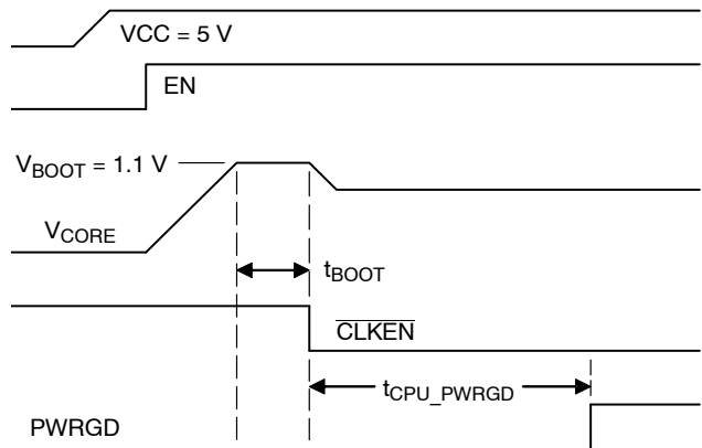
Figure 20. Powerup Sequence of APD3212A/NCP3218A
