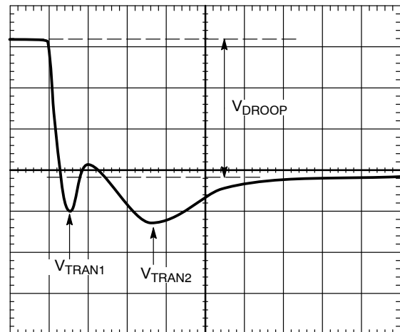
Figure 17. Transient Setting Waveform
