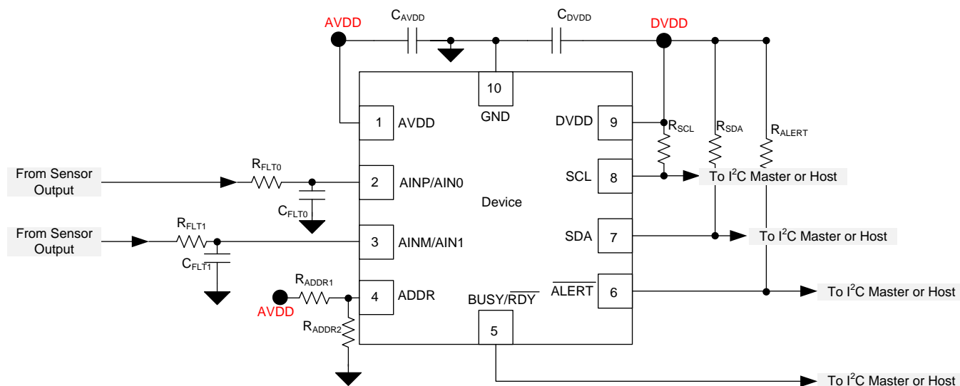
Figure 123. Example Circuit
