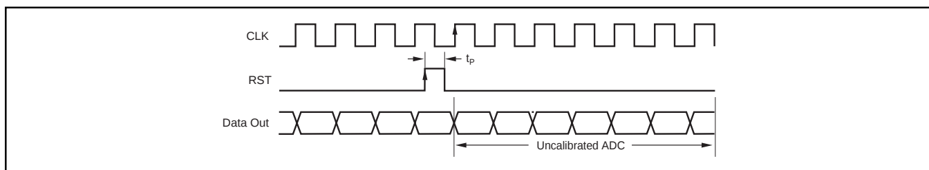
TIMING DIAGRAM 4. Reset Mode Timing.
