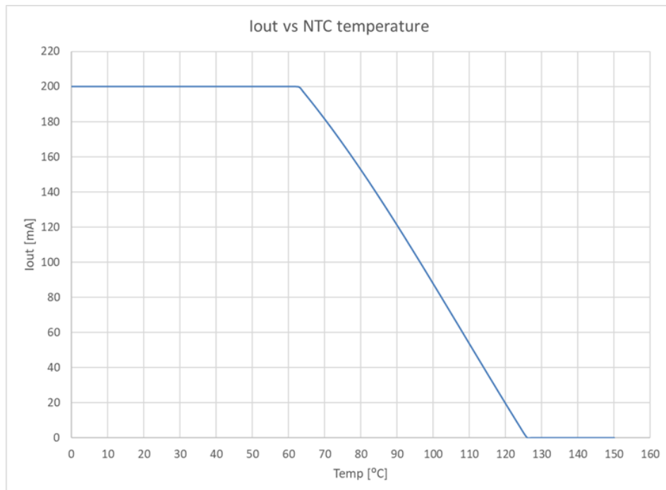
Figure 18. Simulated I_{OUT} vs. NTC temperature
