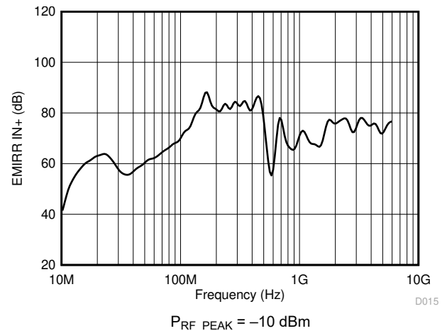
Figure 6-28. EMIRR vs Frequency
