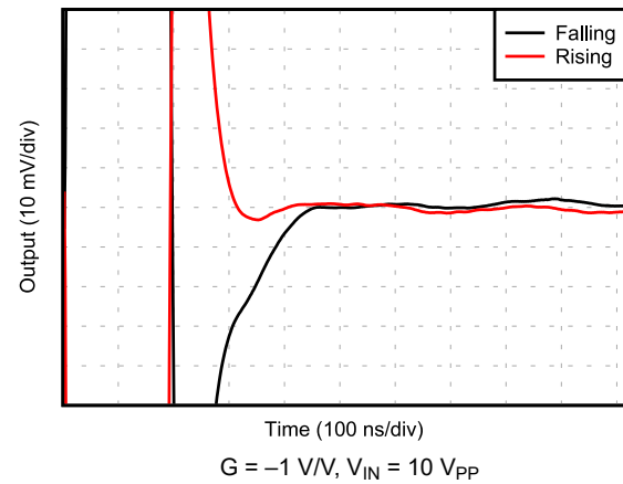
Figure 6-26. Settling Time
