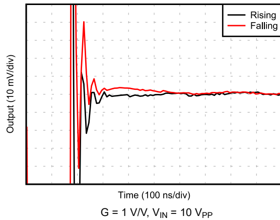
Figure 6-25. Settling Time
