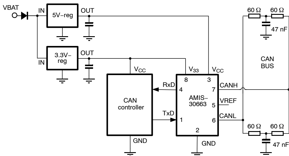
Figure 2. Application Diagram
