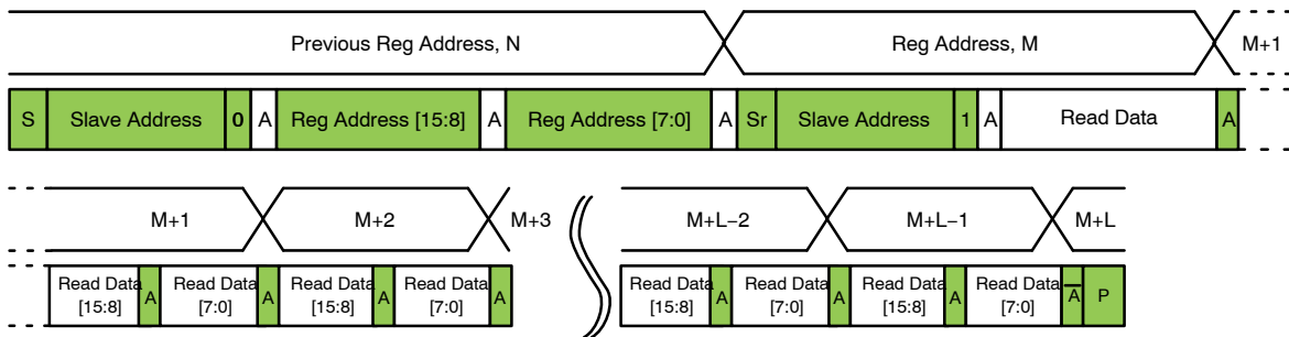
Figure 17. Sequential READ, Start from Random Location
