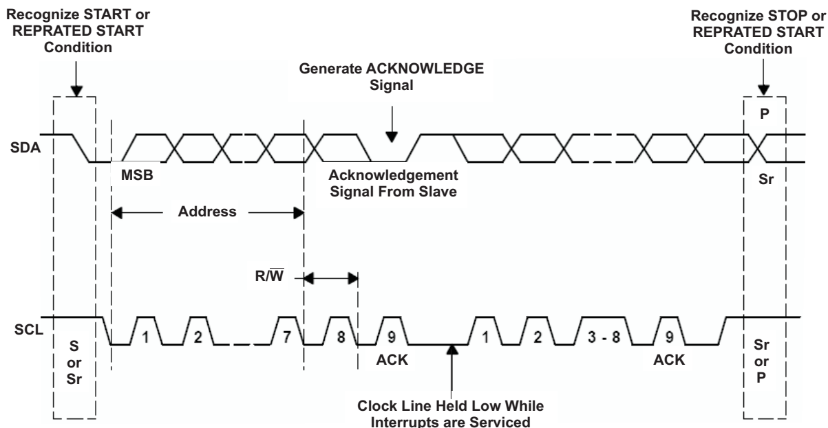
Figure 18. Bus Protocol
