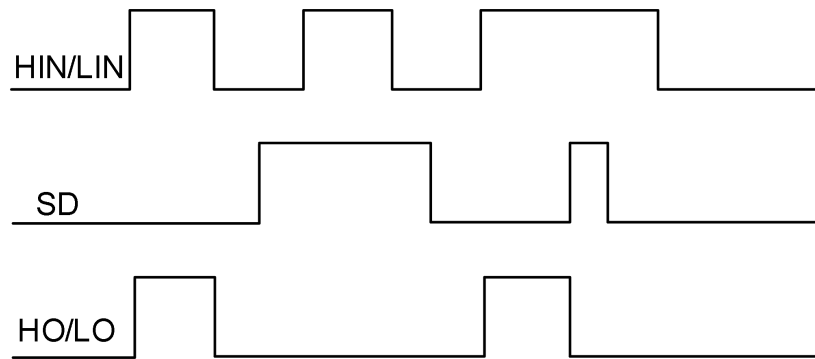
Figure 8-1 IRS2113STR Input and output timing waveform
