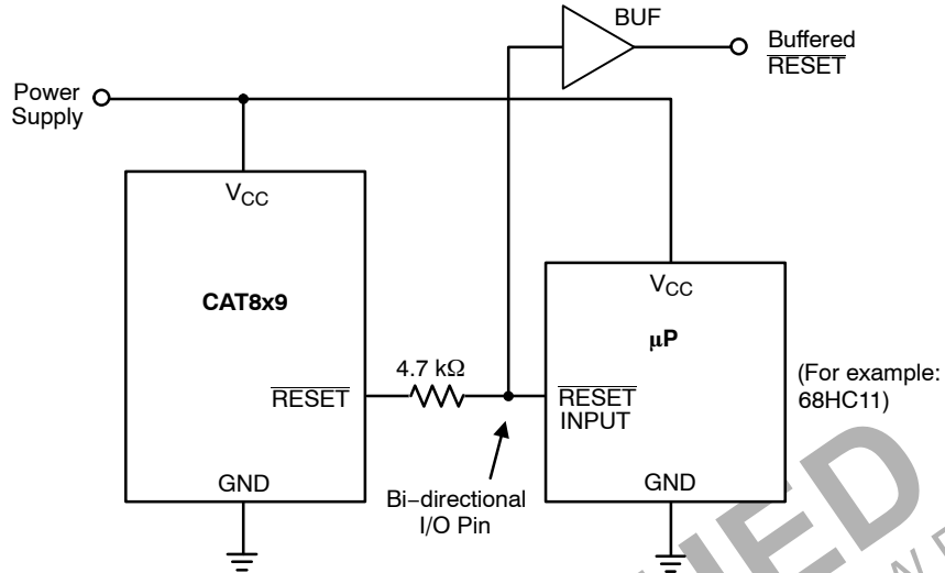
Figure 9. Bi-directional Reset Pin Interfacing
