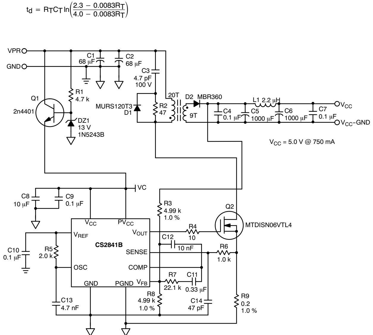
Figure 8. Flyback Application
