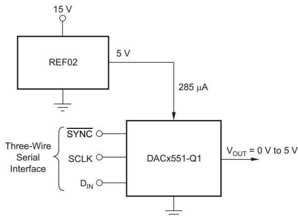
Figure 37. REF02 As a Power Supply to the DACx551-Q1
