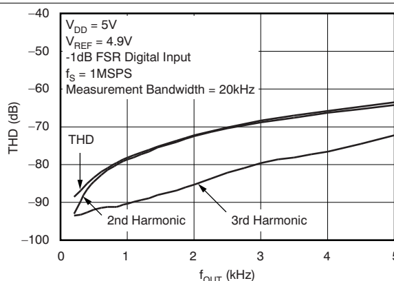
Figure 23. Total Harmonic Distortion vs Output Frequency
